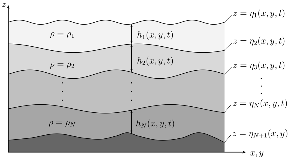
FIGURE 1. The layered model of the ocean. The upper surface of each layer is given by z = \eta_i(x, y, t) , and the layer thickness by h_i(x, y, t) .
