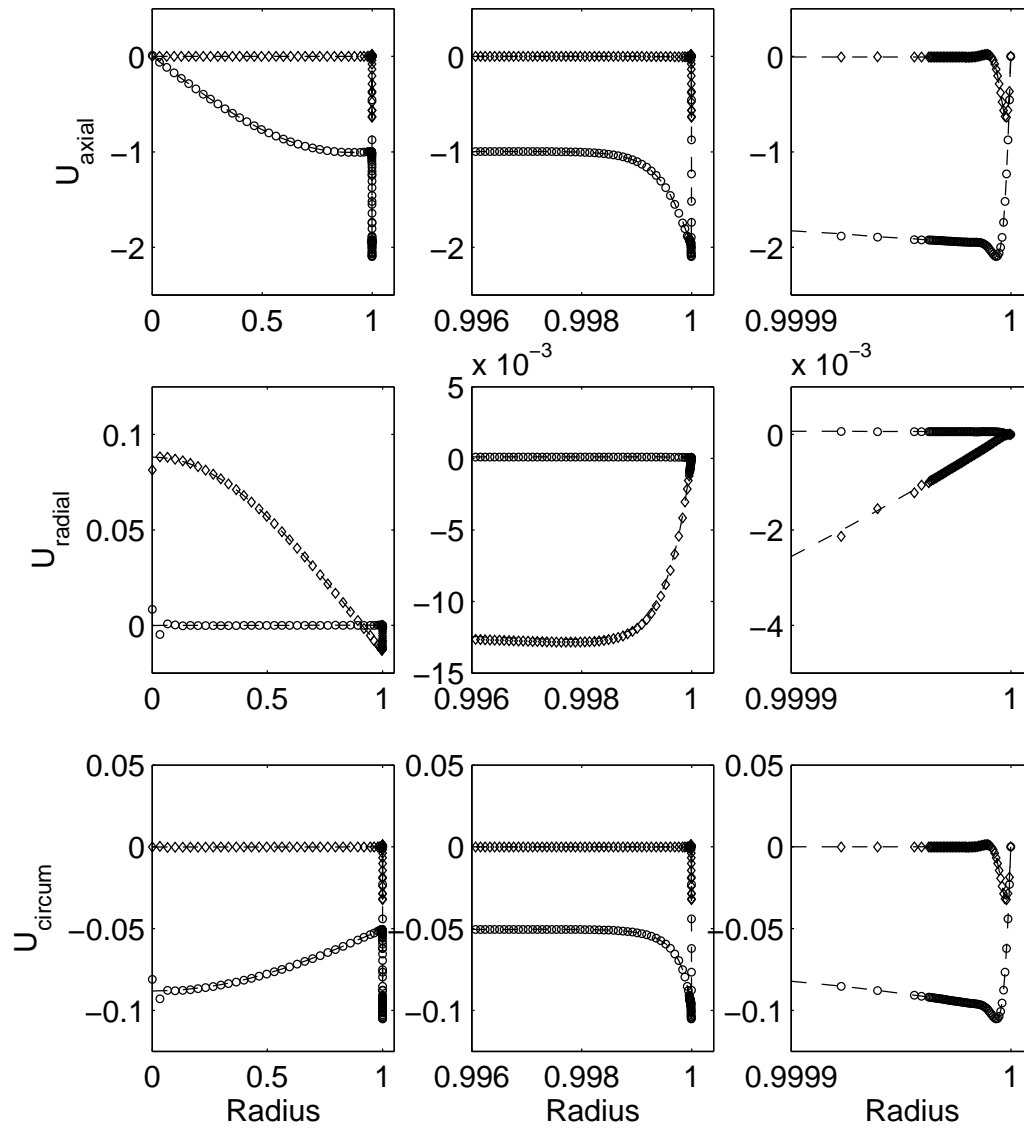
Figure 5: Comparison of numerical (symbol) and asymptotic (line) values for axial, radial and circumferential velocity components in the core, steady boundary and Stokes sublayer.
