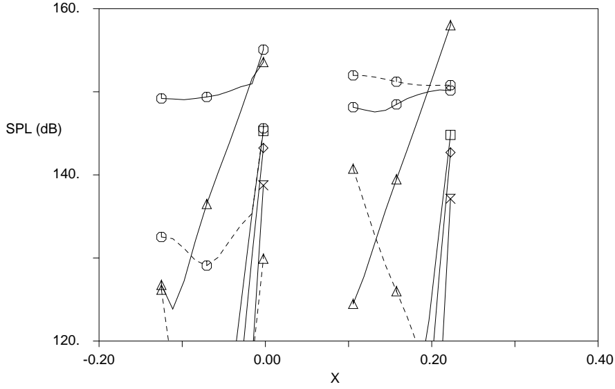
Figure 7: Inviscid annular cascade: amplitude of the first radial harmonic acoustic mode propagating upstream (straight line) and downstream (dashed line) for circumferential Fourier modes -32(\diamond) , -8(\times) , 16(\triangle) , 40(\circ) and 64(\square) .
