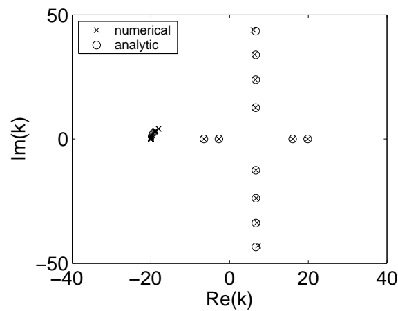
Figure 1: Numerical wavenumbers for inviscid annular duct flow; r_{\text{inner}}/r_{\text{outer}} = 0.5 , M = 0.5 , \omega = 10 , m = 1 .
