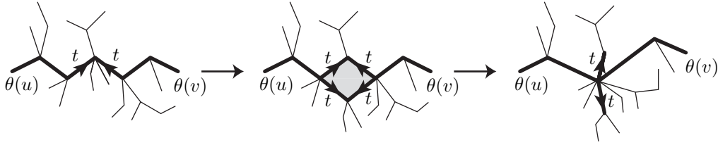
Figure 11: A diamond move.
