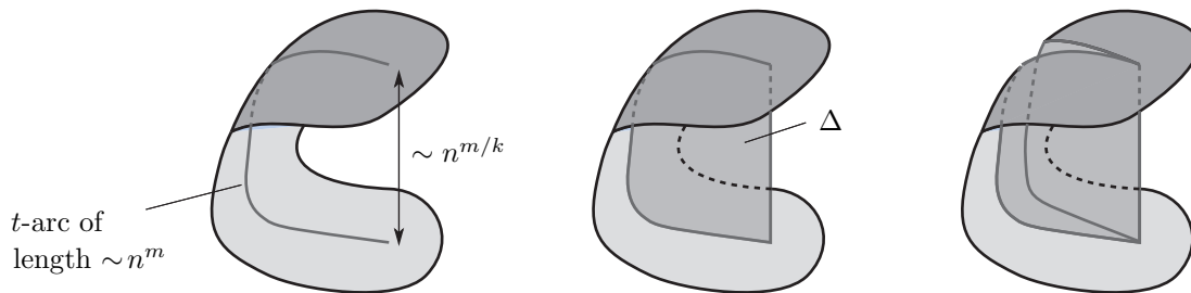
Figure 1: Inserting a shortcut diagram \Delta .
