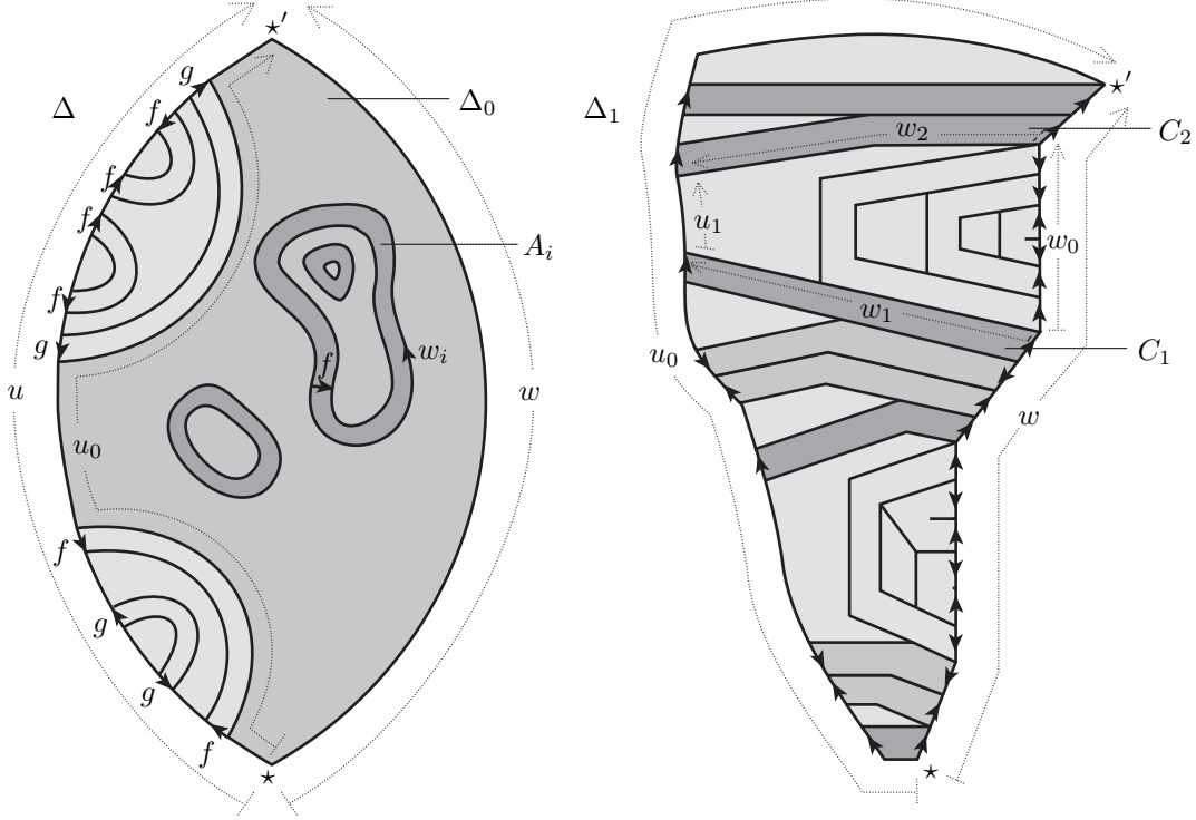
Figure 6: Corridors in the \mathcal{P}_k -van Kampen diagram \Delta .
