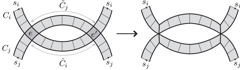
Figure 7: Removing twice-crossing corridors.
