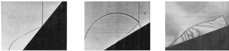
FIGURE 2. Three patterns of shock reflection-diffraction configurations.
