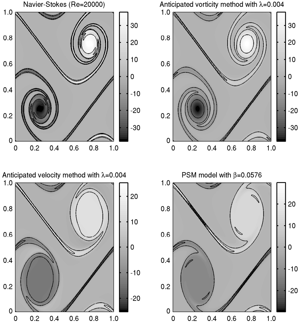
FIGURE 5. The vorticity at the later time t = 1.2 from the same four sets of equations as figure 4.
