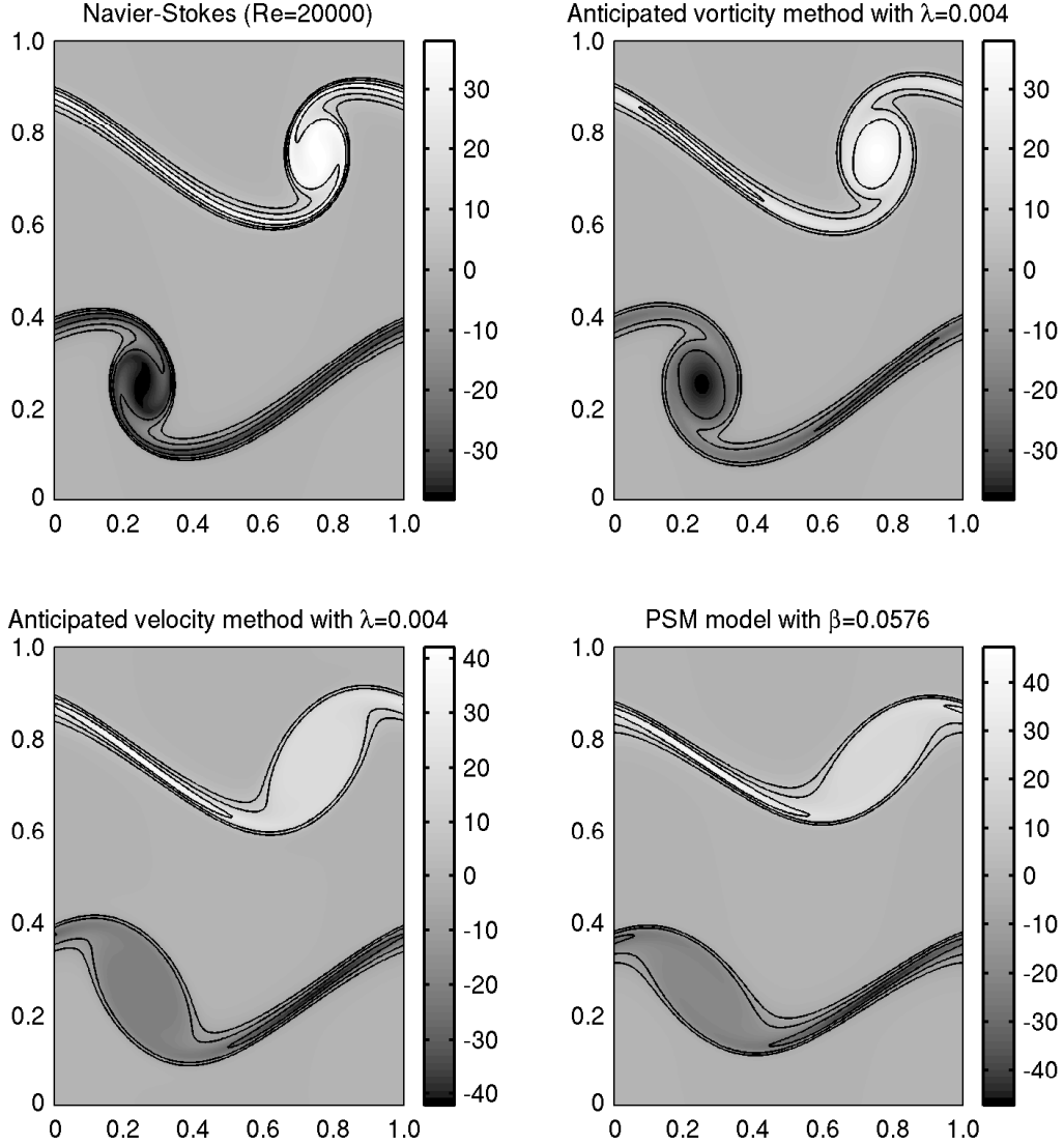
FIGURE 4. The four plots show the vorticity at time t = 0.80 from the unmodified Navier-Stokes equations, the anticipated vorticity method with \lambda = 0.004 , the anticipated velocity method also with \lambda = 0.004 , and the PSM model with \beta = (72/5)\lambda = 0.0576 . All four equations included a linear viscous term corresponding to an initial Reynolds number of 2 \times 10^4 .
