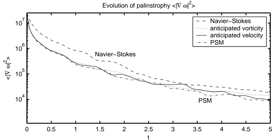
FIGURE 13. Evolution of the palinstrophy \langle |\nabla \omega|^2 \rangle on a logarithmic scale for the same four equations and parameter values as figure 6.
