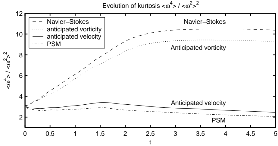
FIGURE 8. Evolution of the kurtosis \langle \omega^4 \rangle / \langle \omega^2 \rangle^2 for the same four equations and parameter values as figure 6.
