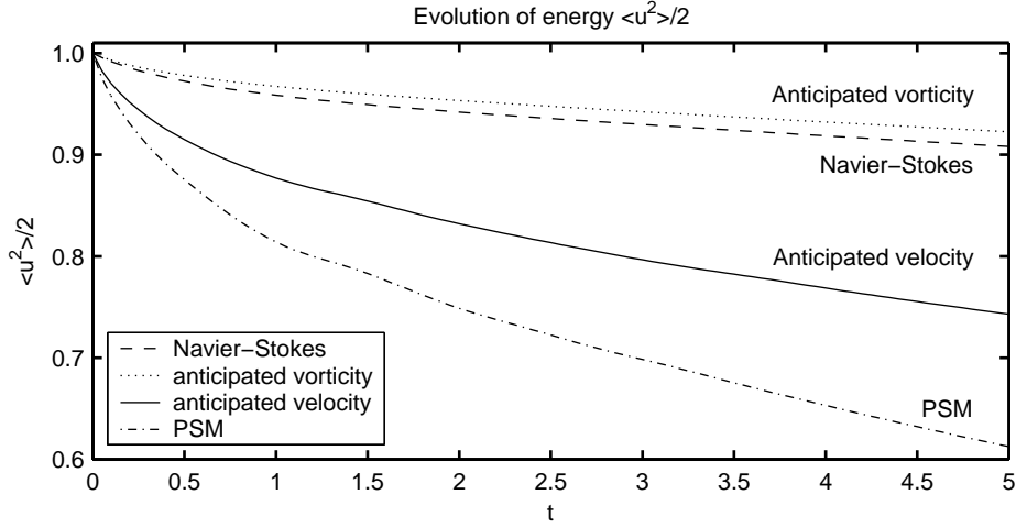
FIGURE 11. Evolution of the energy \langle \frac{1}{2}u^2 \rangle for the same four equations and parameter values as figure 6.
