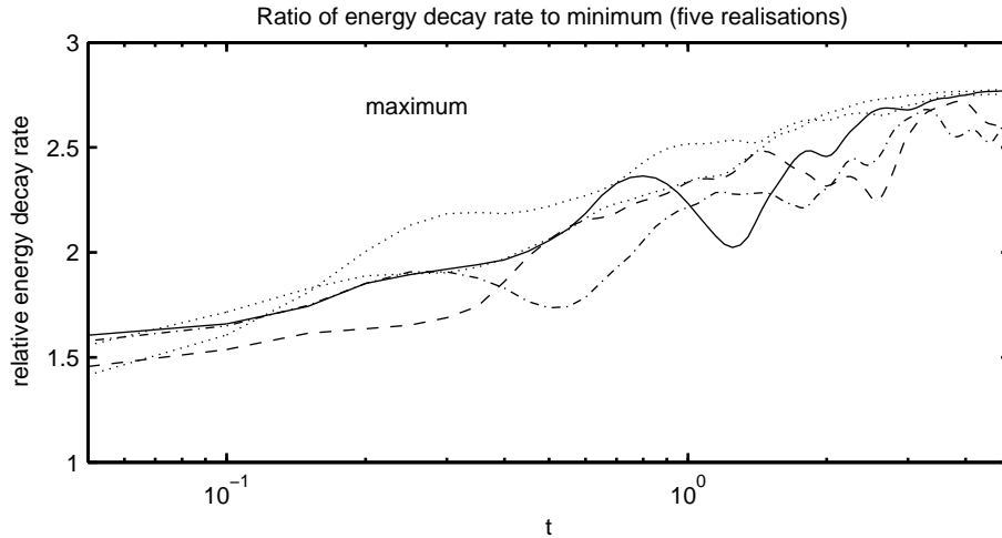
FIGURE 14. Ratio of the energy decay rate in the PSM equation to the minimum given in (5.6) for five different realisations with the same parameter \beta = 0.00576 and initial Reynolds number Re = 10^4 . The upper bound becomes 2.8 times the lower bound in the inviscid limit, and is shown by the horizontal line.
