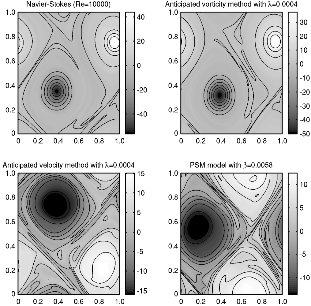
FIGURE 7. The four plots show the vorticity at the later time t = 5.0 for the same four equations and parameter values as figure 6.
