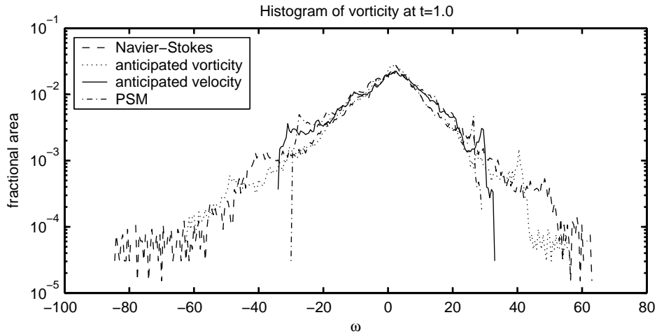
FIGURE 9. Histogram of vorticity values at t = 1.0 for the same four equations and parameter values as figure 6.
