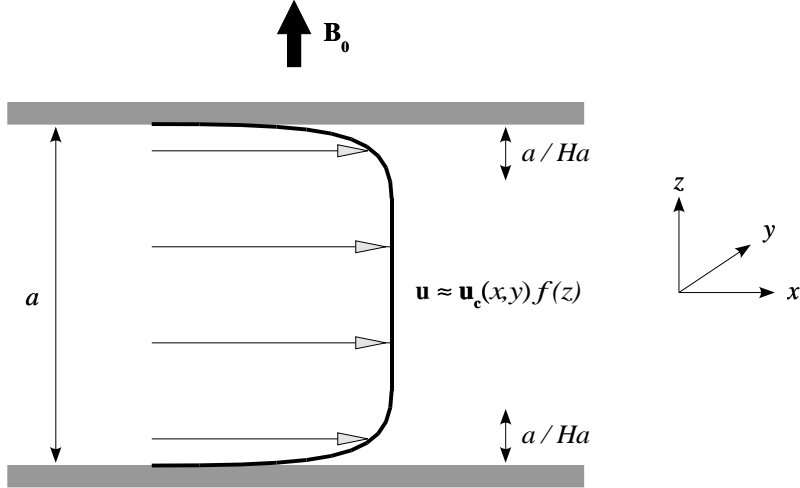
FIGURE 1. Hartmann layers form on walls perpendicular to the imposed magnetic field \mathbf{B}_0 . The core velocity \mathbf{u}_c decays to zero over a distance a/Ha = \sqrt{\rho\eta_*\nu}/B_0 to satisfy the no-slip boundary condition on the walls.
