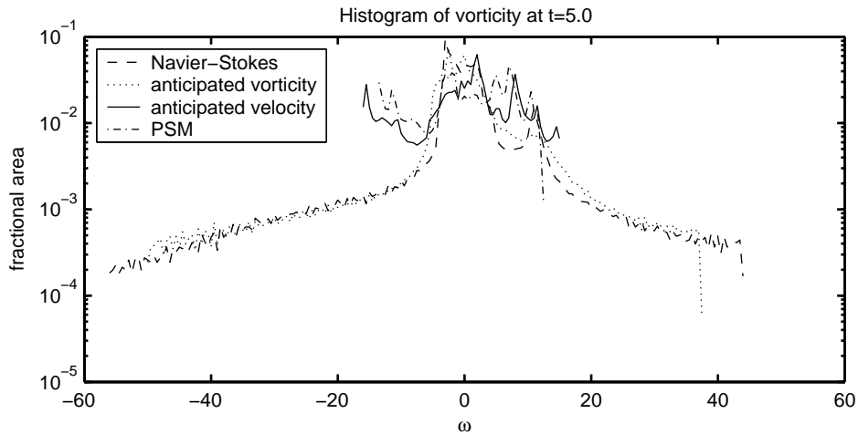
FIGURE 10. Histogram of vorticity values at t = 5.0 for the same four equations and parameter values as figure 6.
