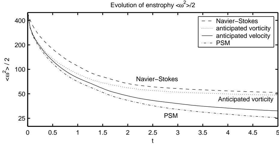
FIGURE 12. Evolution of the enstrophy \langle \frac{1}{2}\omega^2 \rangle on a logarithmic scale for the same four equations and parameter values as figure 6.
