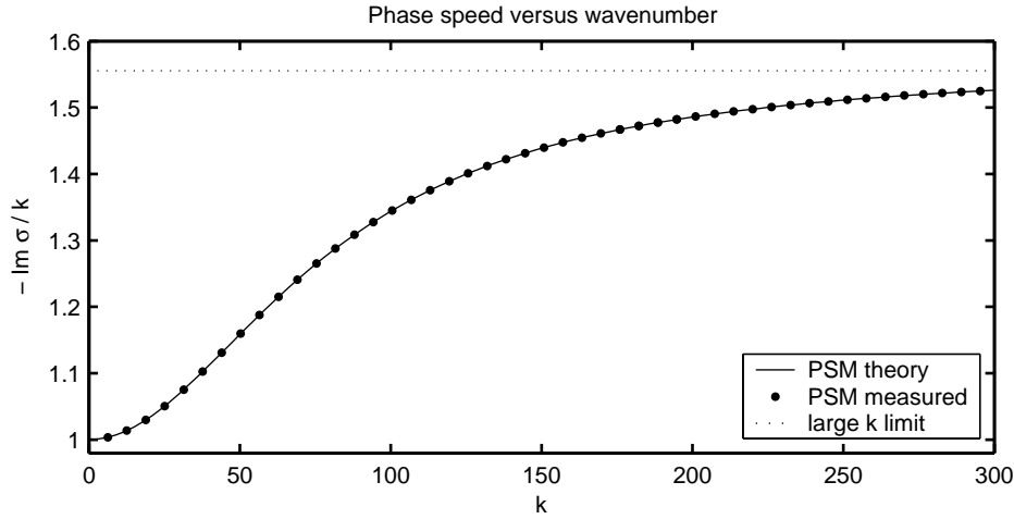
FIGURE 3. Phase speed -\text{Im } \sigma/k versus wavenumber k for the PSM model with U = 1 , \beta = 0.1 , and \nu = 10^{-4} . The solid line is the theoretical prediction from equation (6.1), and the dots are numerical measurements from simulations (see §8.1). The upper dotted line is the large wavenumber limit, -\text{Im } \sigma/k \rightarrow (14/9)U as k \rightarrow \infty . The phase speed remains unchanged for all the explicit methods.
