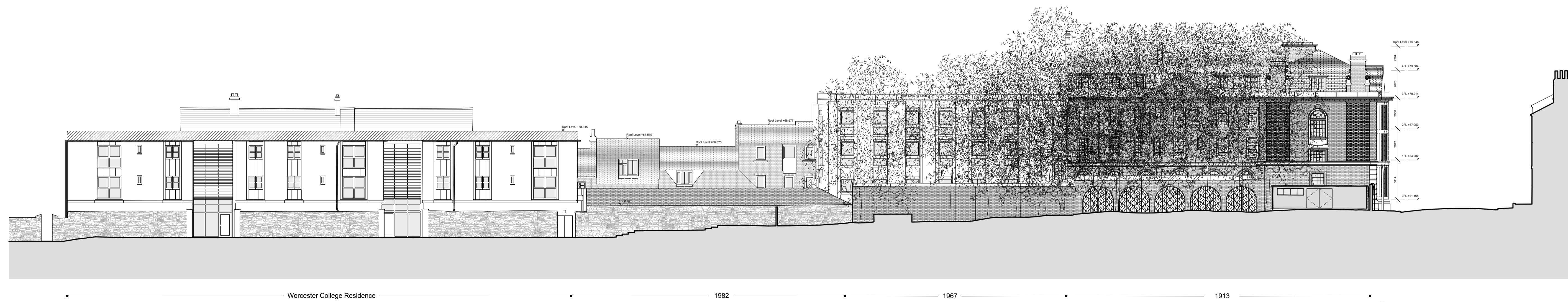
2 1:100 RUSKIN LANE ELEVATION
