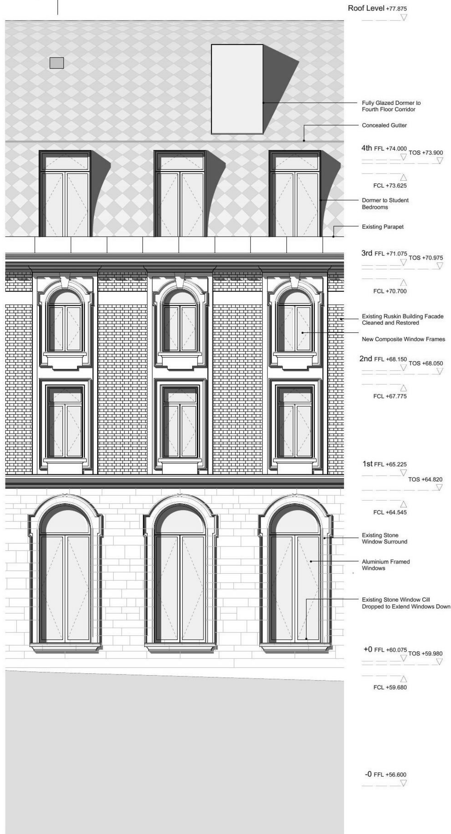
1 DETAILED ELEVATION 02 1:50
