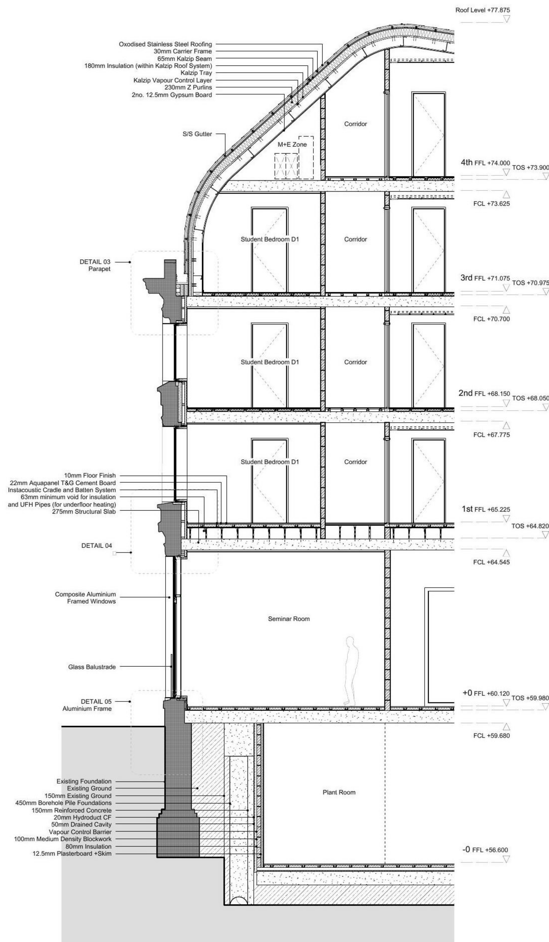
2 DETAILED SECTION 02 1:50
