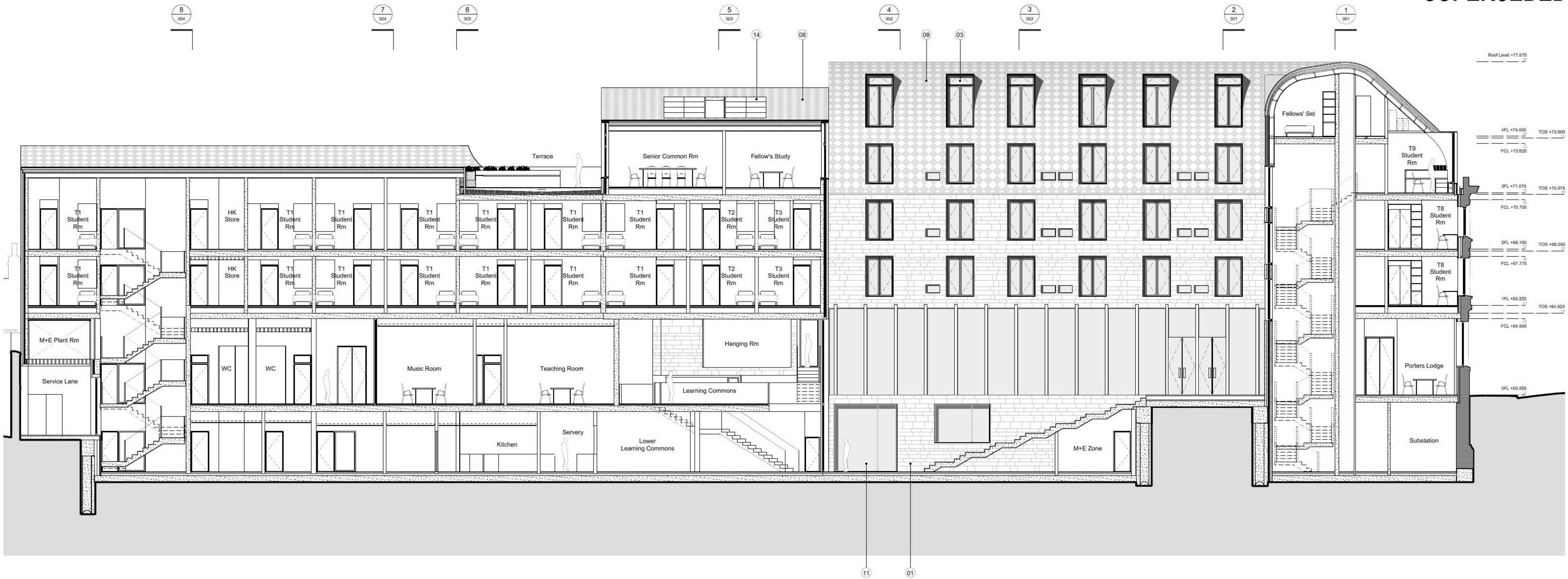
12 LONG SECTION 12
