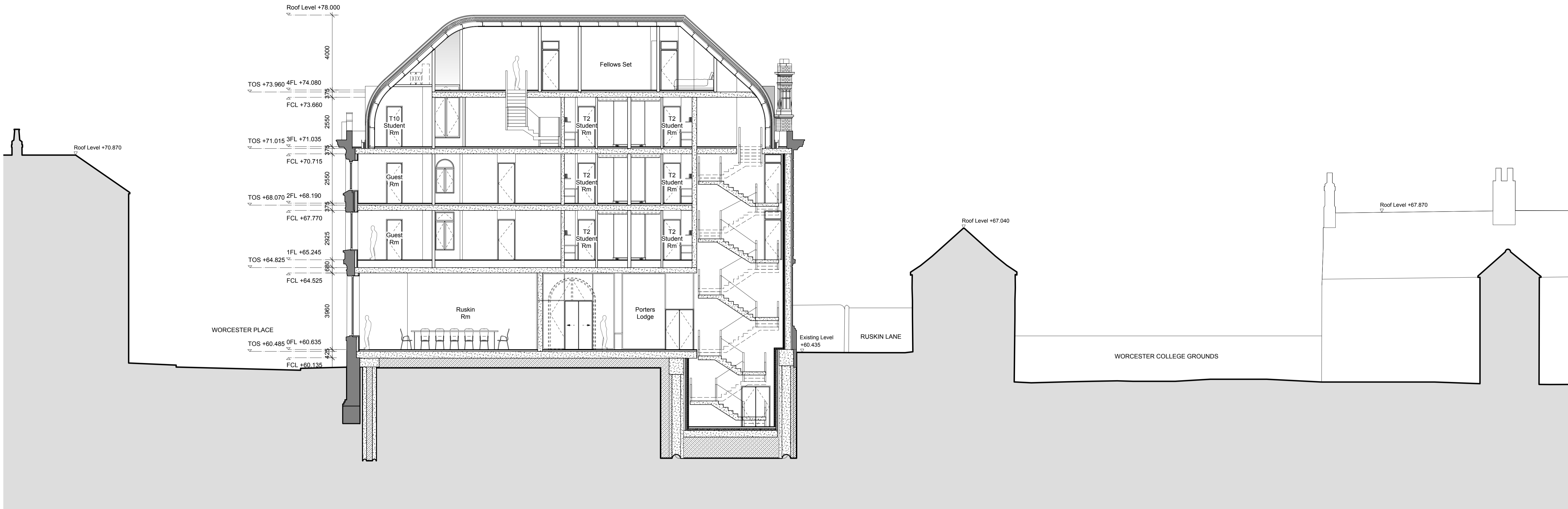
1 CROSS SECTION 1
