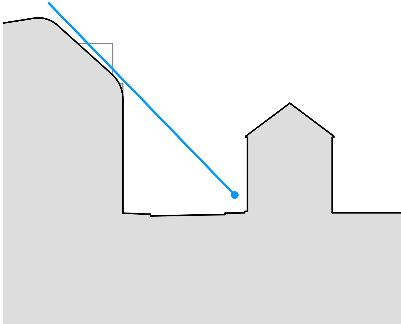
Section D - Planning Proposal
