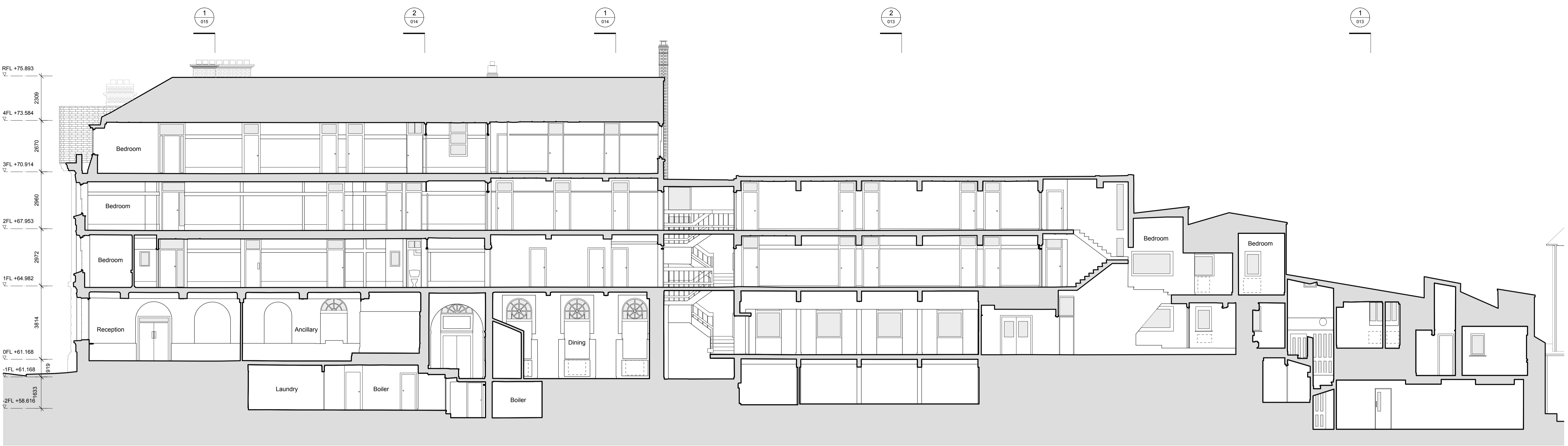
1 SECTION.FF 1:100
