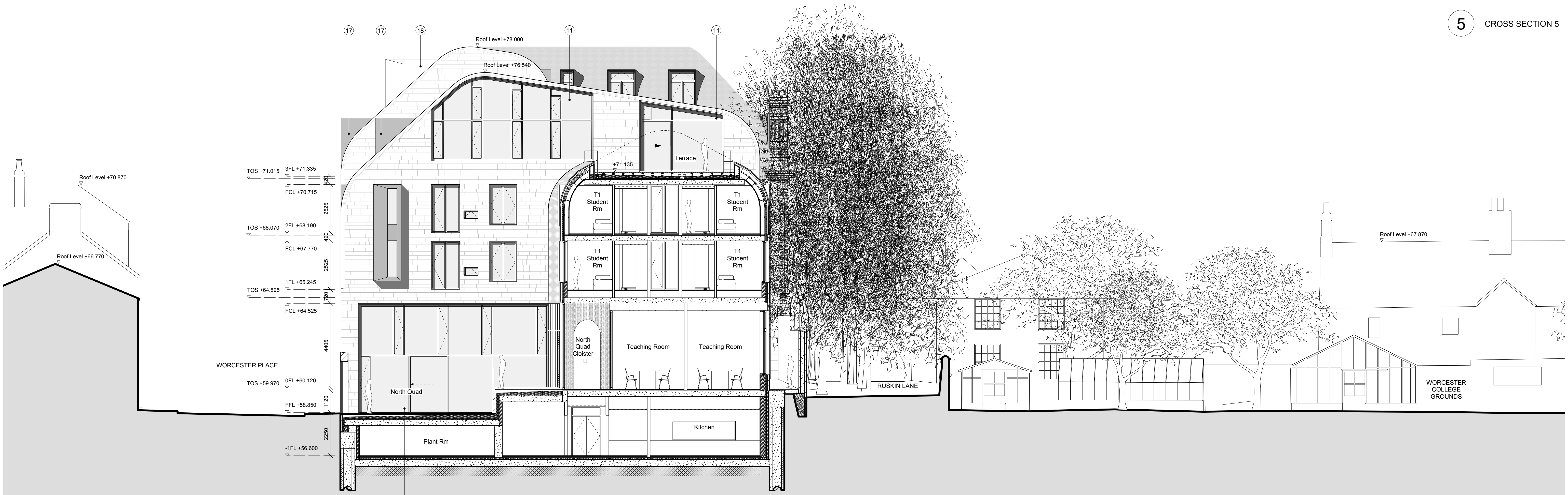
6 CROSS SECTION 6
