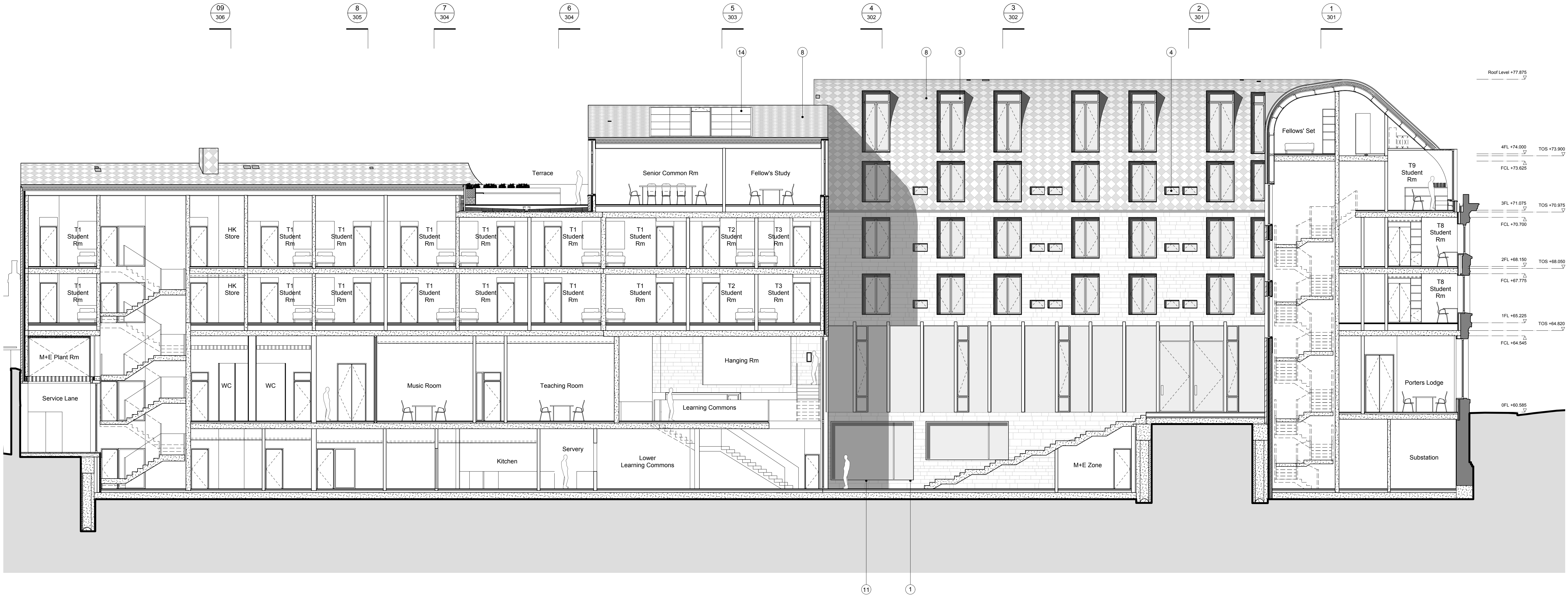
12 LONG SECTION 12
