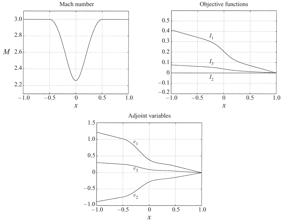
FIGURE 1. Mach number, objective functions and adjoint variables for supersonic flow conditions. M_{\text{in}} = 3 , H_{\text{in}} = 4 , p_{0\text{in}} = 2 .
