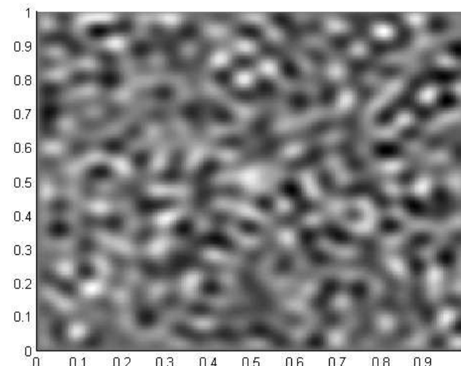
A typical realisation of \kappa for \lambda = 0.001 , \sigma = 1 .
