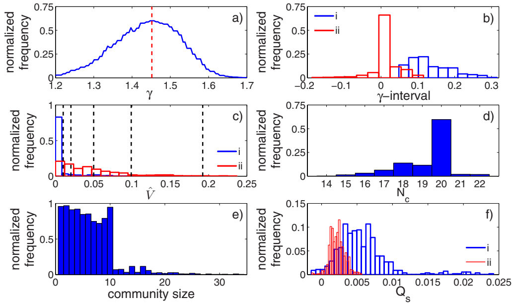
FIG. 2. (Color online) (a) Observed fraction of time steps that the resolution \gamma lies in the main plateau. The vertical line indicates the value \gamma=1.45 , which lies in the largest number of main plateaus and is the resolution at which we investigate the community dynamics. (b) (i) Normalized sampled distribution of the main plateau width and (ii) normalized sampled distribution of the \gamma -distance between the main plateau and \gamma=1.45 . (c) (i) Distribution of normalized variation of information between the community configuration at \gamma=1.45 and the configuration corresponding to the main plateau and (ii) distribution of normalized variation of information between consecutive time steps. The vertical lines give the mean \hat{V} when (left to right) 1, 2, 5, 10, and 20 nodes are randomly reassigned to different communities (averaged over 100 reassignments for each time step). (d) The fraction of time steps at which N_c communities are observed. (e) The fraction of time steps at which a community of a given size is observed. (f) Comparison of the distribution of the scaled energy for (i) market data and (ii) 100 realizations of shuffled data.
