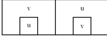
Figure 5: The gadget G'_e
