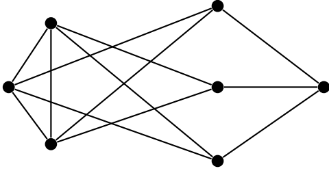
Figure 1: Mycielskian of K_3 ( M_3(1, 1, 1) )
