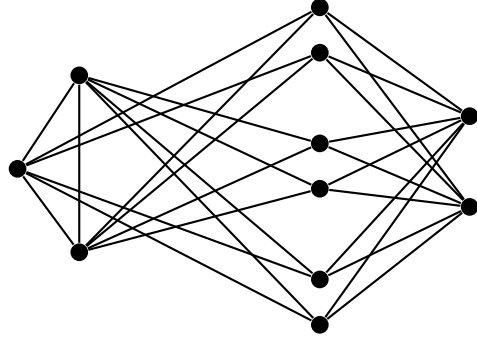
Figure 2: M_3(1, 2, 2)
