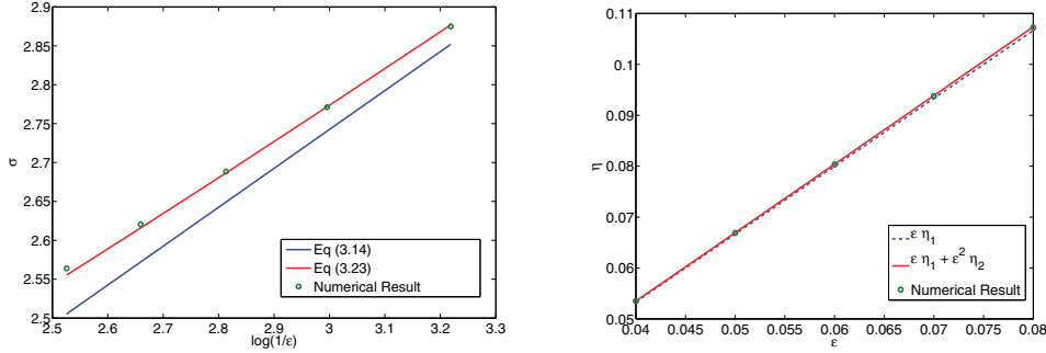
FIG. 2. Comparing the asymptotic and numerical results for (left) the position of the free boundary and (right) the chemical potential, for a range of \epsilon and r_0 = 1/2 .
