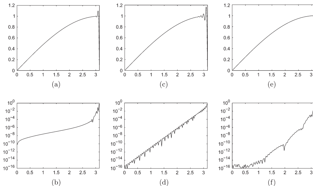
FIG. 3. Recovery of f_1(x) (top) and the approximation error (bottom) from their N = 128 -mode spectral projections. The filter (3.1) was of orders N^{1/4} in (a,b), N^{1/2} in (c,d) and \max(2, \frac{1}{2}(Nd(x))^{1/2}) in (e,f).
