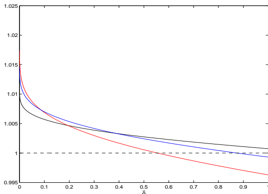
Figure 2: Improvement Ratios for Selected \beta : The ratio \rho_S^{cwx}(\delta, \beta) / \rho_S^{cwx}(\delta; 4) for ( \beta = 3 , red), ( \beta = 3.25 , blue), ( \beta = 3.5 , black).
