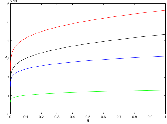
Figure 1: Regions of Strong Equivalence : The region below the curve \rho_S(\delta) is a region of StrongEquiv(A, \ell^1) for A drawn from the Gaussian ensemble; (\rho_S^{cwx}(\delta; 4) , red), (\rho_S^{bt}(\delta) , black), (\rho_S^{fl}(\delta) , blue), (\rho_S(\delta) , green).
