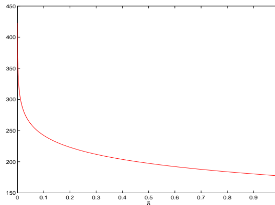
Figure 3: Proportionality Constants : the curve 1/\rho_S^{cwx}(\delta; 4) which provides the constant of proportionality between the required number of measurements and the sparsity level.
