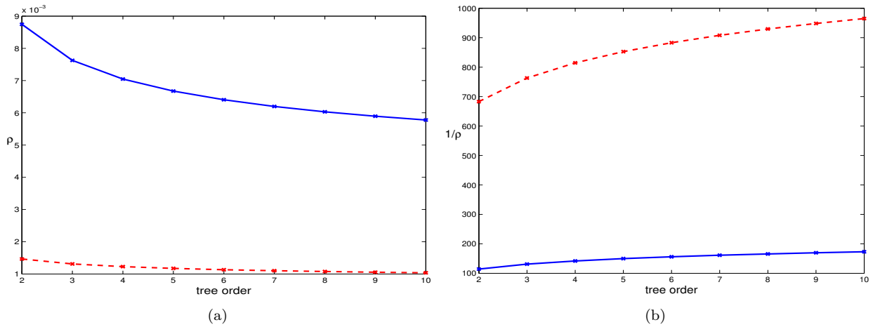
Figure 2: (a) Critical \rho -values for different tree orders from tree-based RIP analysis: ITP – unbroken; NITP – dashed. (b) Corresponding oversampling factors (reciprocals of \hat{\rho} ).
