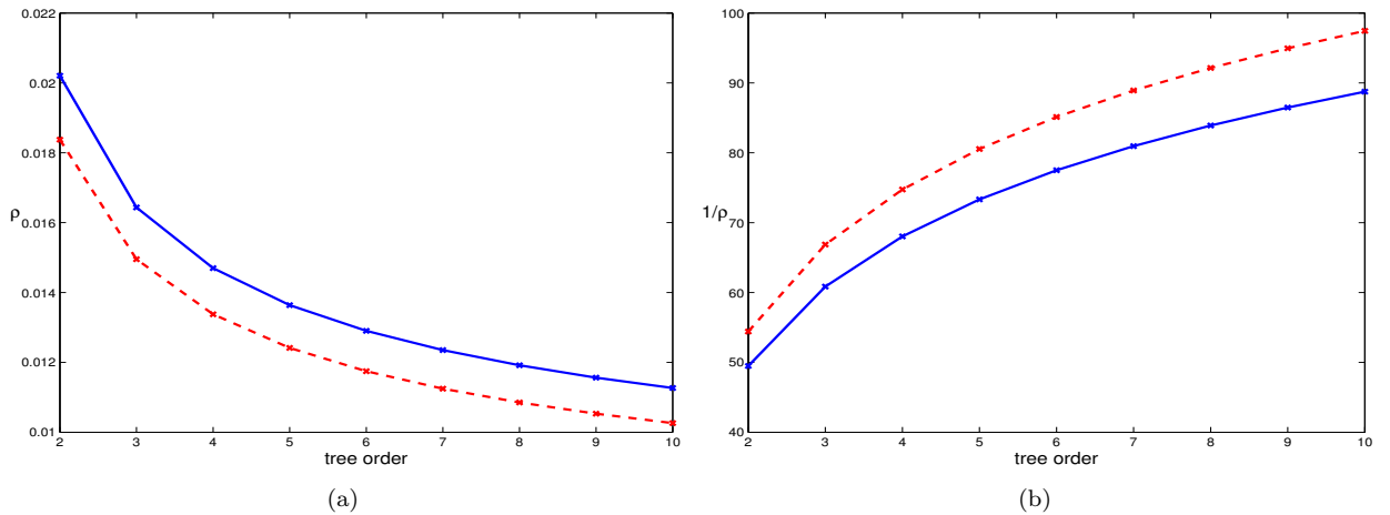
Figure 5: (a) Critical \rho -values for different tree orders from stable point analysis: ITP – unbroken; NITP – dashed. (b) Corresponding oversampling factors (reciprocals of \hat{\rho} ).
