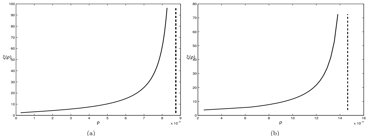
Figure 7: Plot of the stability factor \xi(\rho) from stable point analysis for binary trees: (a) ITP; (b) NITP.
