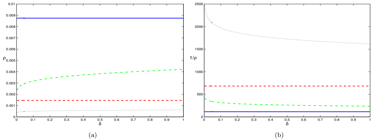
Figure 3: (a) Phase transitions from RIP analysis in the (\delta, \rho) framework for binary trees (ITP – unbroken; NITP – dashed) and non-tree-based (IHT – dash-dot; NIHT – dotted). (b) Corresponding inverses of the phase transition.
