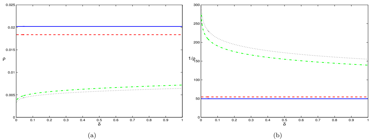
Figure 6: (a) Phase transitions from stable point analysis in the (\delta, \rho) framework for binary trees (ITP – unbroken; NITP – dashed) and non-tree-based (IHT – dash-dot; NIHT – dotted). (b) Corresponding inverses of the phase transition.
