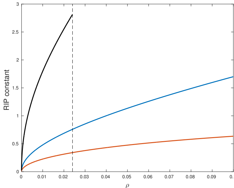
Figure 1: A comparison of \mathcal{TL}(\rho) (red), \mathcal{TU}(\rho) (blue) and \mathcal{TR}(\rho) (black) where defined, for \rho \in (0, 0.1) .
