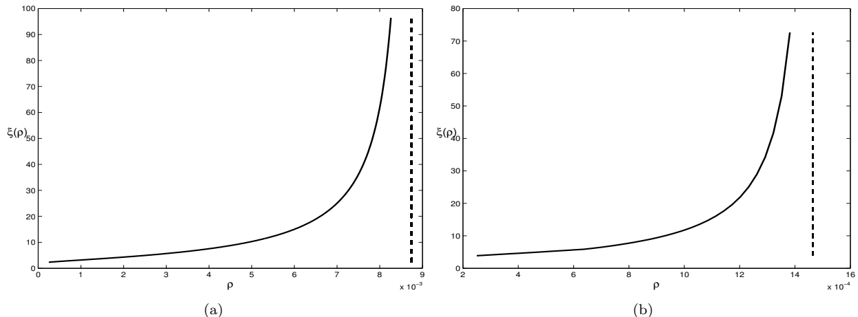
Figure 4: Plot of the stability factor \xi(\rho)/[1 - \mu(\rho)] from tree-based RIP analysis for binary trees: (a) ITP; (b) NITP.
