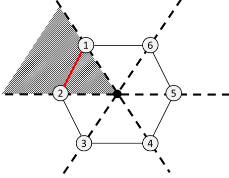
Figure 1: The Euclidean embedding of C_6 .
