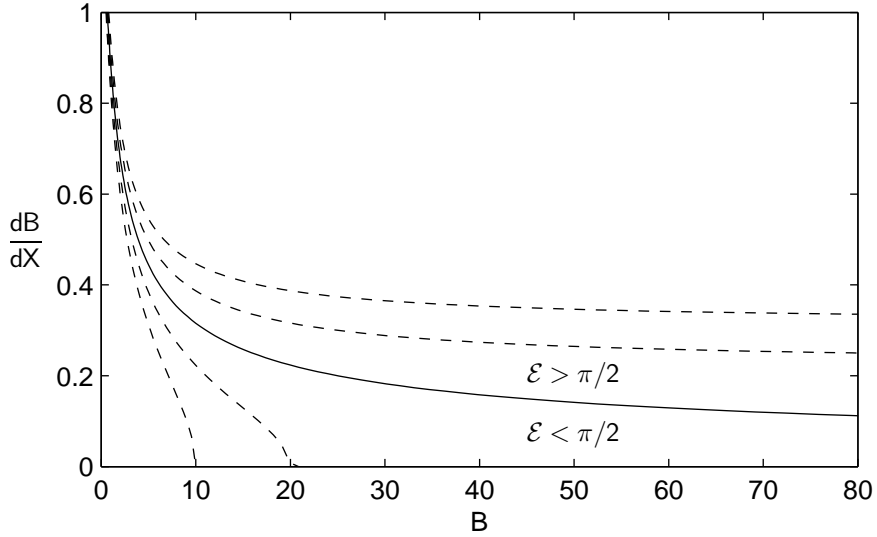
FIGURE 6. Phase plane for the ODE in (8.8). The trajectory with \mathcal{E} = \pi/2 (shown solid) is the only trajectory for which dB/dX \rightarrow 0 as B \rightarrow \infty . The other trajectories shown dotted have \mathcal{E} = \pi/2 \pm 0.05 and \mathcal{E} = \pi/2 \pm 0.1 .
