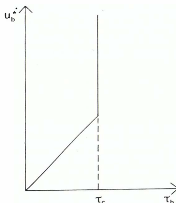
Fig. 2. Cavitational sliding law.
