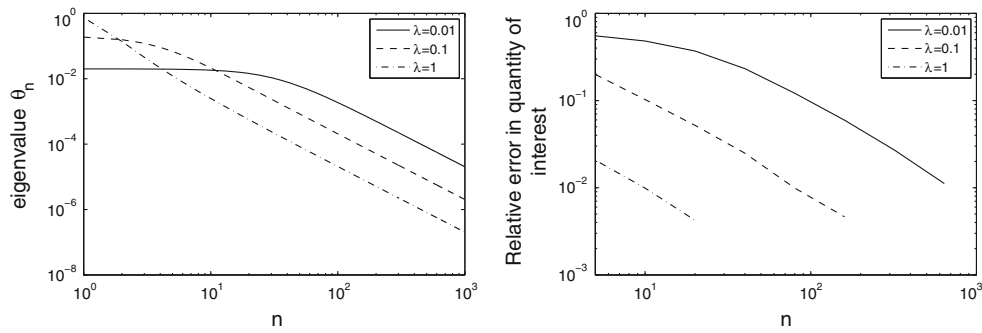
Fig. 1 Left plot of the KL eigenvalues in decreasing order as a function of their index, for different choices of the correlation length \lambda and for d = 1 . Right corresponding relative error (or bias) |\mathbb{E}[k_{\text{eff}}(Z)] -
