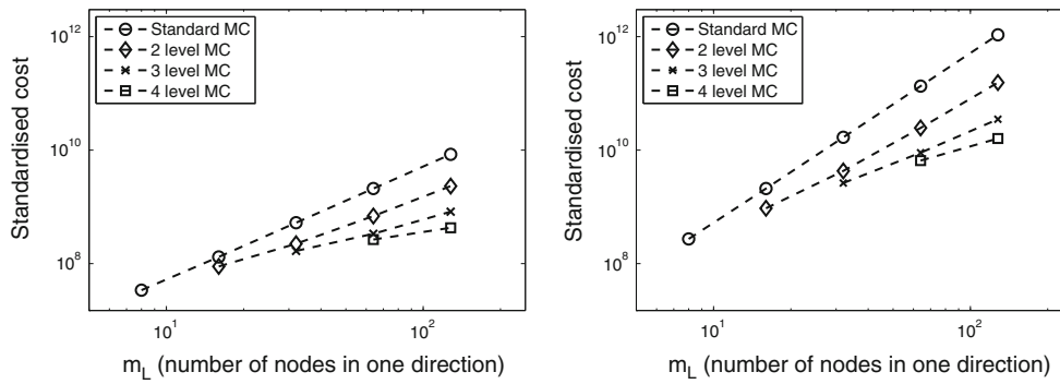
Fig. 4 Plots of the standardised cost (scaled by 1/C^* ) versus m_L for a fixed tolerance of \delta = 10^{-3} for the maximum standard deviation of the MLMC estimator for \mathbb{E}[k_{\text{eff}}] for \lambda = 0.3, \sigma^2 = 1, m_{\text{KL}} = 1400 assuming \gamma = 1 (left plot) and \gamma = 1.5 (right plot)
