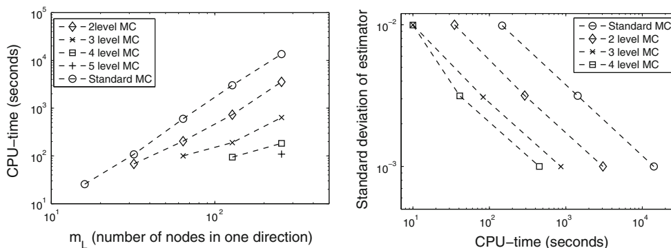
Fig. 7 Same plots as in Figs. 4 and 5 for \lambda = 0.1 , \sigma^2 = 1 , m_{KL} = 500 , but using actual CPU time in seconds to quantify the cost (Matlab implementation running on a 3 GHz Intel Core 2 Duo E8400 proces-
