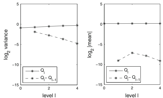
Fig. 6 Plots of \mathbb{V}[Q_\ell] and \mathbb{V}[Y_\ell] (left plot), as well as \mathbb{E}[Q_\ell] and \mathbb{E}[Y_\ell] (right plot) in the case \lambda = 0.3, \sigma^2 = 1, m_{\text{KL}} = 1400 in 2D, with m_0 = 4 and Q = -k \frac{\partial p}{\partial x_1} at the centre of the domain
