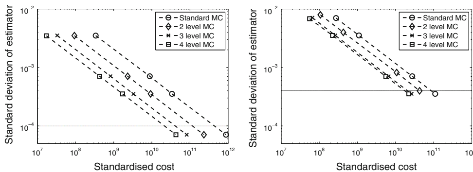
Fig. 5 Same test case as in Fig. 4. Standard deviation of the MLMC estimator \hat{Q}_L^{ML} versus the standardised computational cost for fixed m_L = 128 . The horizontal line represents the estimated spatial discretisation error on this grid. Quantities of interest: \mathbb{E}[k_{\text{eff}}] (left plot) and \mathbb{E}\left[-k \frac{\partial p}{\partial x_1}\right] at the centre of the domain (right plot)
