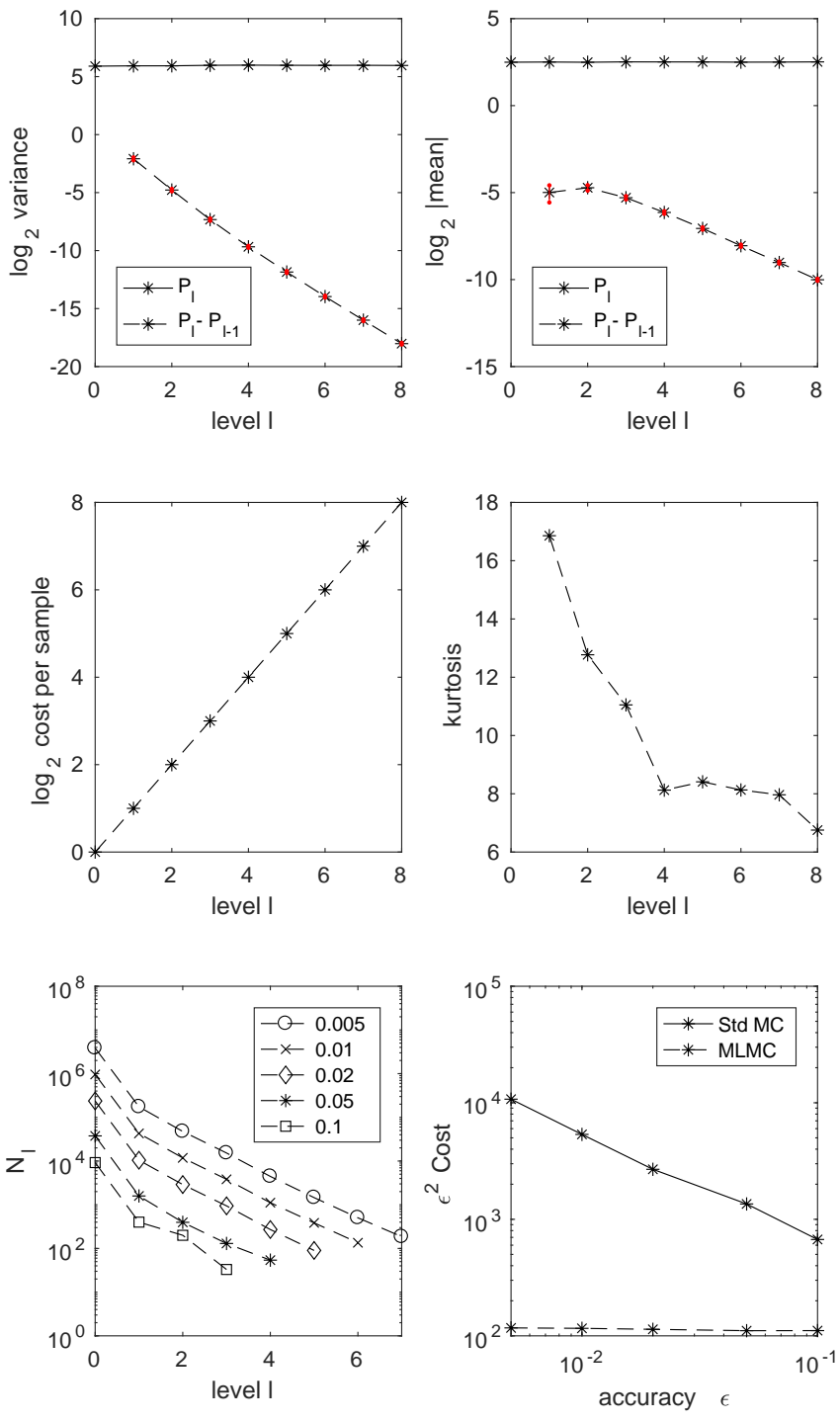
Figure 2: Asian call
