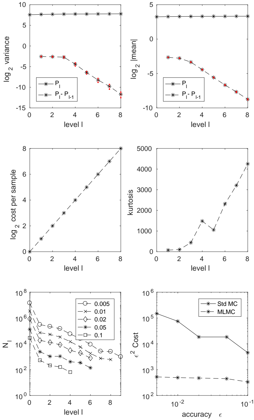
Figure 5: Barrier call
