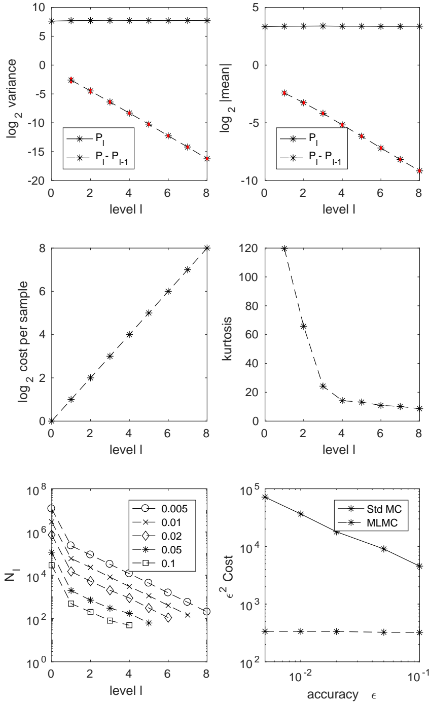
Figure 1: European call
