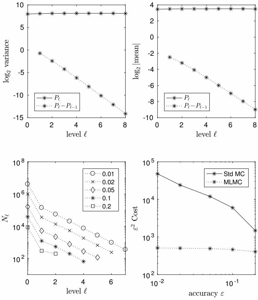
Figure 1: European basket call based on geometric Brownian motion
