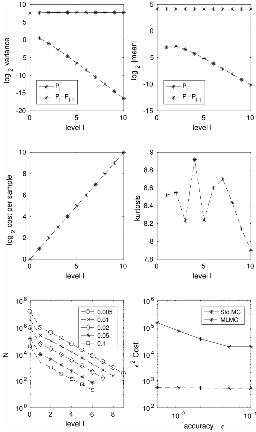
Figure 13: Lookback call
