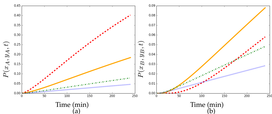
Figure 11: Infection risk versus time in an 8\text{m} \times 8\text{m} \times 3\text{m} classroom for an infectious person breathing in a case of very poor ventilation (red dashed), poor ventilation (orange solid), ASHRAE recommended minimum ventilation for classrooms (green dot-dashed) and a ventilation better than the ASHRAE recommended minimum (blue dotted), using (2.16) and (2.19), with parameter values as given in Tables 1 and 6. (a) Evaluated at Position A:(5,4) . (b) Evaluated at Position B:(8,8) . Here, \mathcal{R} = 1 , which corresponds to breathing.
