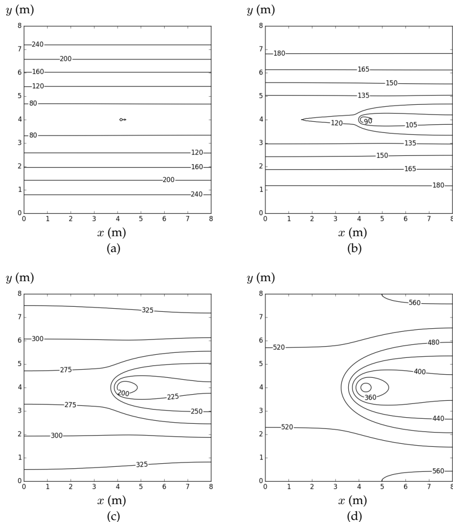
Figure 13: ‘Time to probable infection’ (TTPI) due to an infectious person talking at the centre of a 8\text{m} \times 8\text{m} \times 3\text{m} room from (2.16) and (2.19), with parameter values from 1 and 6: (a) very poor ventilation, (b) poor ventilation (c)ASHRAE recommended ventilation for classrooms (d) a ventilation better than the ASHRAE recommended minimum. \mathcal{R} = 10 for talking.
