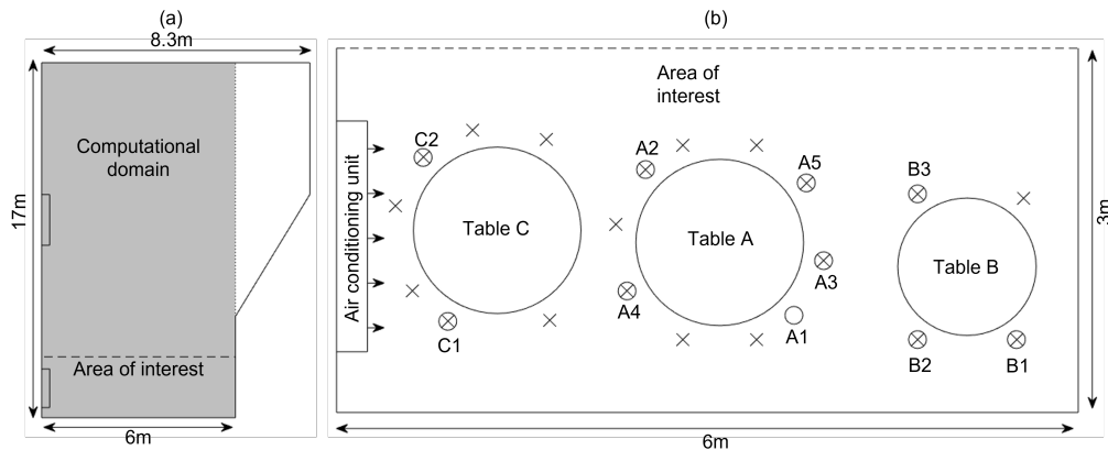
Figure 4: (a) The 6m × 17m computational domain, shown in grey, over which we run our model as a simplified version of the Guangzhou restaurant [31]. (b) The area of interest contains the ‘recirculating zone’ in which 7-9 people were infected by A1, the infectious person. The circled X denotes an infected person and X denotes a person who was not infected.
