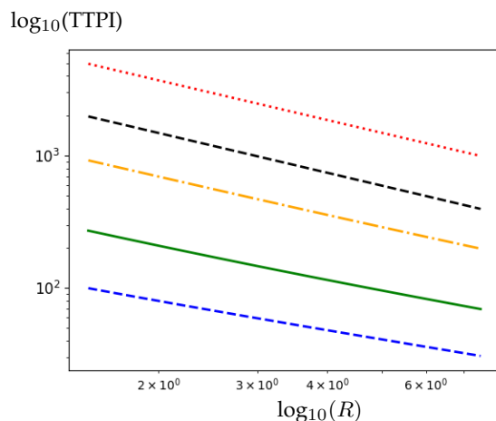
Figure 16: Log–log plot of the TTPI versus R , in rooms with poor ventilation, evaluated at 1m downwind from the infectious person, from solving Equations (2.16) and (2.19). The black dashed line represents an infinite room; the red dotted line represents a convention centre ( 68\text{m} \times 105\text{m} ); the orange dot-dashed line represents an auditorium ( 15\text{m} \times 30\text{m} ); the green solid line represents a classroom ( 8\text{m} \times 8\text{m} ); and the blue dashed line represents a personal office ( 4\text{m} \times 4\text{m} ). All other parameter values are given in Table 1.
