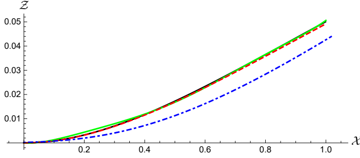
Fig. 5 Comparison of the prediction of the deflection of a soft fiber wrapping around a 0.25 mm radius particle in 0.1 mM NaCl for the fiber configuration given by the solution to the reduced model for small-deflection prestressed states (14) (red dashed) and the experimental data (green solid). The match between the data and the theory is excellent. We also show in blue dot dashed the prestressed state and in black the solution to the full model presented in the Model Equations section (see Supplementary Information† for details). The difference between the two theories is almost discernible, supporting the use of the simplified model (14).
