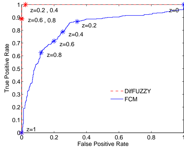
Figure B.13 DifFUZZY and FCM curve for the ‘half moons’ dataset [ M = 300 , h = 1 , corresponding to the left, green moon in Figure 4(a)] (see online version for colours)
