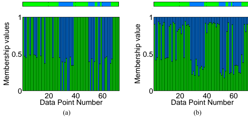
Figure B.10 (a) DifFUZZY membership values for the Leukaemia dataset ( M = 11 ) (b) FCM membership values (see online version for colours)
