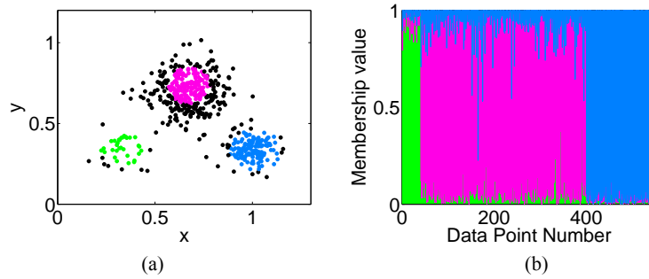
Figure B.2 ‘Globular clusters’ dataset (a) FCM HCT-plot, z = 0.9 (b) FCM membership values for this dataset (see online version for colours)
