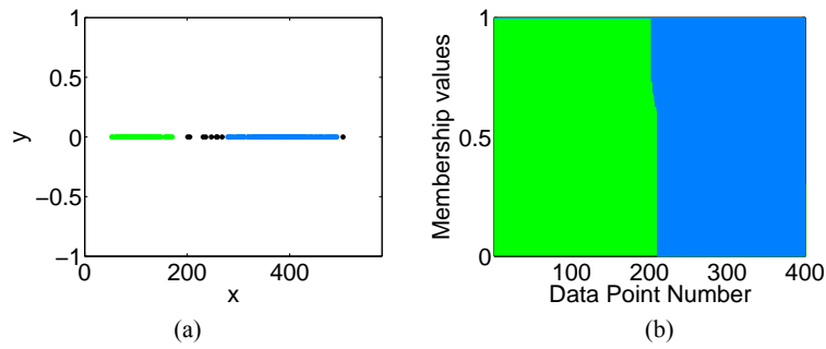
Figure B.6 Dataset obtained by sampling a stochastic dynamical system (a) DifFUZZY HCT-plot, z = 0.9 ( M = 180 ) (b) DifFUZZY membership values ( M = 180 ) (see online version for colours)
