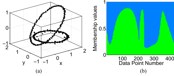
Figure B.4 ‘Interlaced rings’ dataset (a) FCM HCT-plot, z = 0.9 (b) FCM membership values (see online version for colours)
