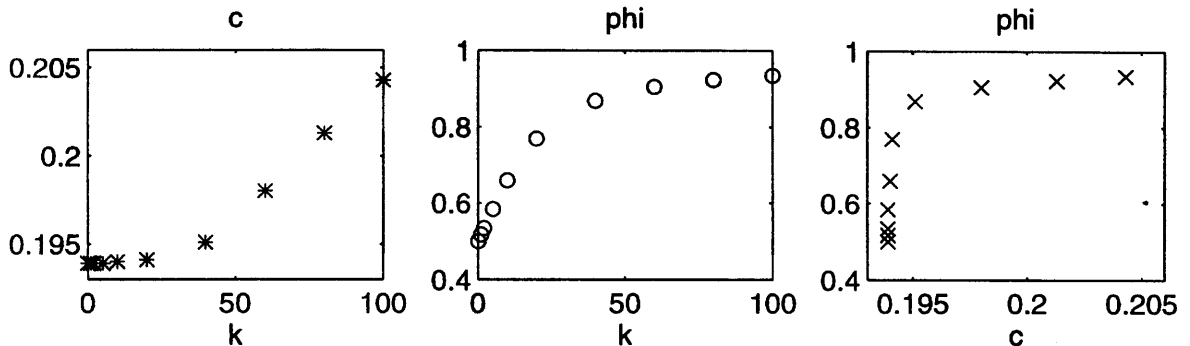
FIGURE 6 Numerical solutions of equations (10)–(12) for k = 0, 1, 2, 5, 10, 20, 40, 60, 80 and 100 from which the wave speed c (left: *) and steady-state value of m_1 (i.e. \phi ; middle: o) are calculated. Also shown is the relationship between \phi and c (right: x). Parameter values (except k ) as in Figure 4. An extended spatial domain is used in these simulations to allow long-time evolution of the wave speed. The theoretical minimum wave speed, c_{\min} \approx 0.197 , is predicted by linear analysis of travelling wave solutions (see text). These results show that the wave speed ( c ) and extent of scarring (given by \phi ) both increase with the alignment rate parameter ( k ), the latter relationship being the more sensitive. Note the very fine resolution of the axis for c , which confirms our result in the main text that c is approximately independent of k .
