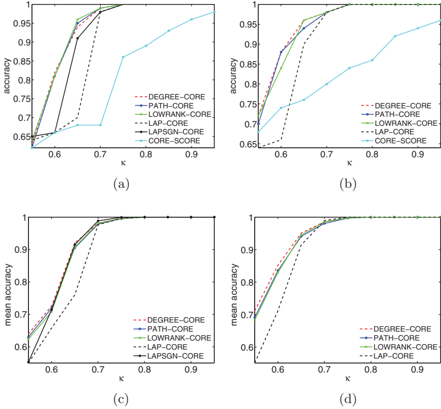
FIGURE 10. Comparison of the methods for graphs with n = 100 vertices generated by a core-periphery block model with edge probabilities \mathbf{p} = (p_{cc}, p_{cp}, p_{pp}) = (\kappa, \kappa, 1 - \kappa) for \kappa \in \{0.55, 0.60, \dots, 0.95\} . We show comparisons for the following situations: (a) without knowledge of \beta , single experiment; (b) with knowledge of \beta , single experiment; (c) without knowledge of \beta , averaged over 100 experiments; and (d) with knowledge of \beta , averaged over 100 experiments.
