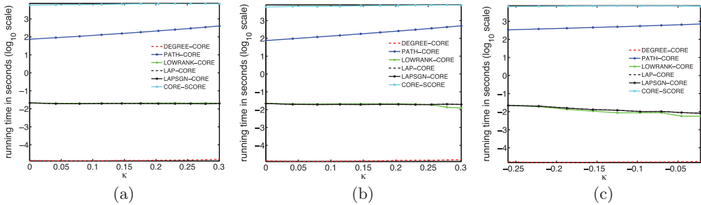
FIGURE 13. Comparison of the computation times (in seconds and on a \log_{10} scale) for all methods and for three synthetic graph ensembles: (a) C_1(n, \beta, p, \kappa) , n = 100 , \beta = 0.5 , p = 0.25 ; (b) C_2(n, \beta, p, \kappa) , n = 100 , \beta = 0.5 , p = 0.25 ; and (c) G(p_{cc}, p_{cp}, p_{pp}) with \mathbf{p} = (p_{cc}, p_{cp}, p_{pp}) = (\kappa, \kappa, 1 - \kappa) .
