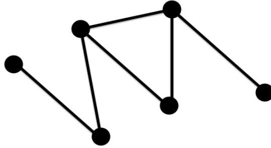
Figure 2: An undirected and unweighted network.
