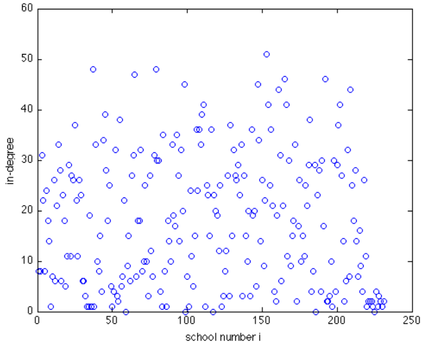
Figure 3: A plot of in-degree against each vertex i , and names of schools are classified in Appendix.
