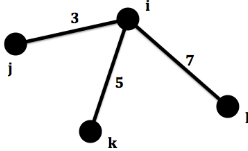
Figure 1: An undirected network.
