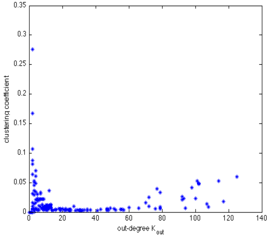
Figure 8: Clustering coefficient against out-degree.
