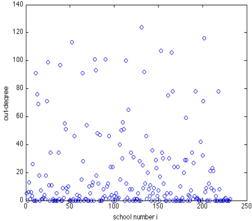
Figure 5: A plot of out-degree against each vertex i
