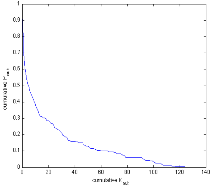
Figure 6: Cumulative degree distribution for out-degree
