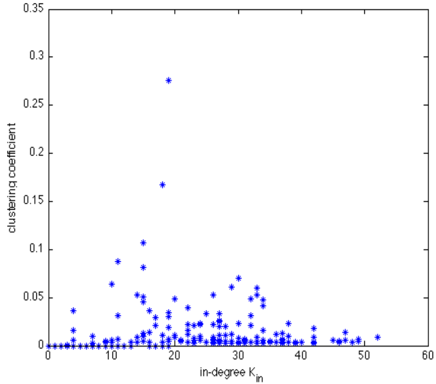
Figure 7: Clustering coefficient against in-degree.
