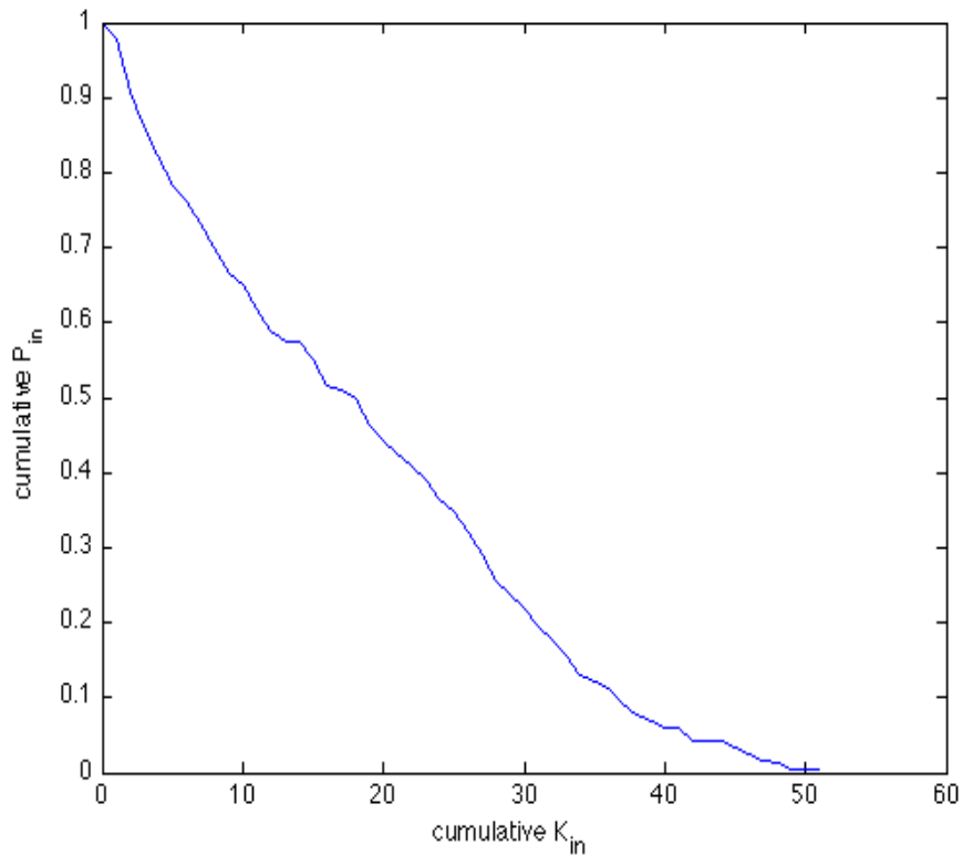
Figure 4: Cumulative degree distribution for in-degree
