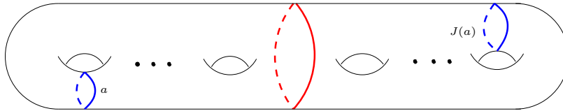
Figure 4: The involution J = -\text{Id} in \mathbb{R}^3 .
