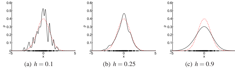
Fig. 2 Kernel density estimate for N = 100 agents, which are placed according to a normal distribution with different bandwidths h . Crosses along the x -axis represent the agents, the dashed line is the underlying Gaussian probability density function and the solid line is the generated estimate by (15).
