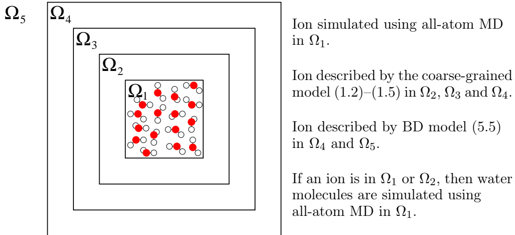
Figure 3. Schematic of multiscale set up. Note that the schematic is drawn in two spatial dimensions to enable better visualization, but all models are formulated and simulated in three spatial dimensions.
