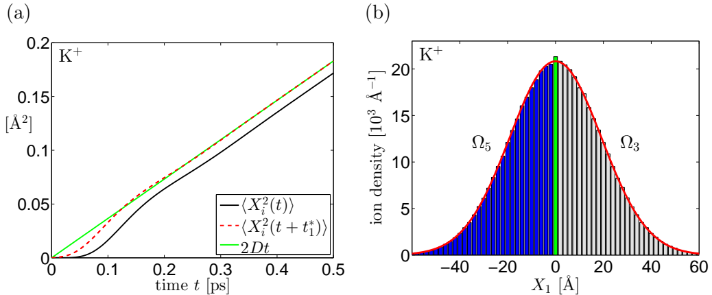
Figure 2. (a) Comparison of the coarse-grained model (1.2)–(1.5) and BD description (1.1) for \text{K}^+ ion. The mean square displacement computed by solving 10 ODEs (3.3)–(3.6), (3.9), (3.11)–(3.14) and (3.16) with zero initial conditions (black solid line). The same curve shifted by the value of t_1^* is plotted as a red dashed line. (b) Test of accuracy of the multiscale approach in \Omega_3 \cup \Omega_4 \cup \Omega_5 for \text{K}^+ ion. Histogram obtained by simulating 10^6 ions over time 10^3 ps is compared with the analytical result (5.6) (red solid line). Grey bars show the ion density in \Omega_3 , the green bar shows the ion density in \Omega_4 and blue bars show the ion density in \Omega_5 . Parameters are given in Tables 1 and 3.
