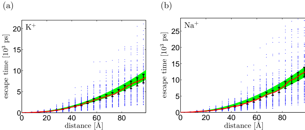
Figure 5. Escape time \mathcal{T}(r) to reach distance r from the origin computed by the multiscale method. We consider (a) \text{K}^+ ion; and (b) \text{Na}^+ ion. We plot escape times for individual realizations (blue points), the mean escape time estimated from 100 realizations (red solid line) and the theoretical 95% confidence interval (6.7) (green area). We use \omega = 10 in (6.2).
