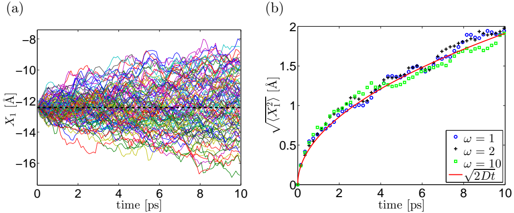
Figure 4. (a) One hundred realizations of a multiscale simulation of K^+ ion initiated at [-L/2, 0, 0] . We plot X_1 coordinate as a function of time. Ion is described by all-atom MD for X_1 \geq -L/2 and by the coarse-grained model (1.2)–(1.5) for X_1 < -L/2 . The boundary between \Omega_1 and \Omega_2 is visualized using the black dashed line. We use \omega = 1 in (6.2). (b) The mean square displacement in the first coordinate of K^+ ion simulated in \Omega_1 \cup \Omega_2 and computed as the average of 100 realizations for \omega = 1 (blue circles), \omega = 2 (black crosses) and \omega = 10 (green squares).
