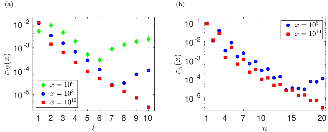
FIGURE 1. (a) Relative errors calculated by (4.1) for x = 10^6 , x = 10^8 and x = 10^{10} .
