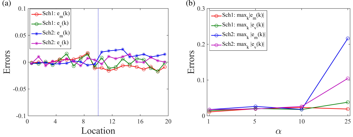
Fig. 4 (a) Errors e_m(k) and e_v(k) given by Equation (4.1) are computed at time 50s. (b) The maximum absolute values of the errors e_m(k) and e_v(k) given by Equation (4.1) are computed at time 50s with a static boundary and different values of \alpha . The maximum value of the errors is taken over all region, \Omega . Red and green lines are relative errors of the means and standard deviations between the analytic solution of the Markov chain model and Scheme 1 . Blue and purple lines are relative errors between the Markov chain model and Scheme 2 .
