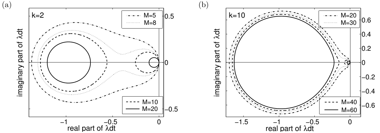
Figure 5: (a) The regions of absolute stability of P_k^M methods for k = 2 and M = 5 (dot-dashed line), M = 8 (dotted line), M = 10 (dashed line) and M = 20 (solid line). (b) The regions of absolute stability of P_k^M methods for k = 10 and M = 20 (dot-dashed line), M = 30 (dotted line), M = 40 (dashed line) and M = 60 (solid line).
