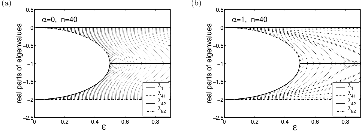
Figure 8: (a) Graph of real parts of eigenvalues of matrix \mathcal{B} for n = 40 and no signal gradient in the environment, i.e., S'_0 = S'_1 = \dots S'_n = 0 . The eigenvalues are real for \varepsilon \in [0, 0.5] and there is a spectral gap between \lambda_{41} and \lambda_{42} . (b) Graph of real parts of eigenvalues of matrix \mathcal{B} for signal given by (3.27) with \alpha = 1 and for n = 40 .
