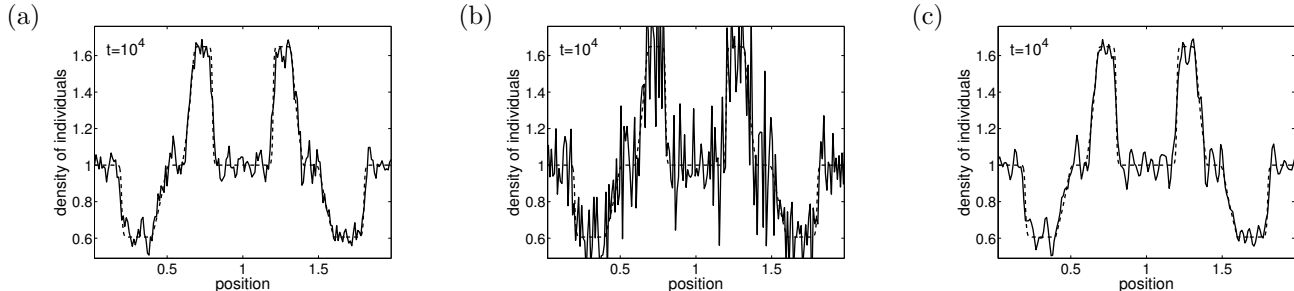
Figure 15: Plots of the density of individuals at time t = 10^4 for the same cumulative distribution function as in Figure 14, using different expressions for computing the discretized density. (a) formula (5.9); (b) formula (5.10); (c) formula (5.11). We also plot the solution of the corresponding macroscopic moment equations (dashed line).
