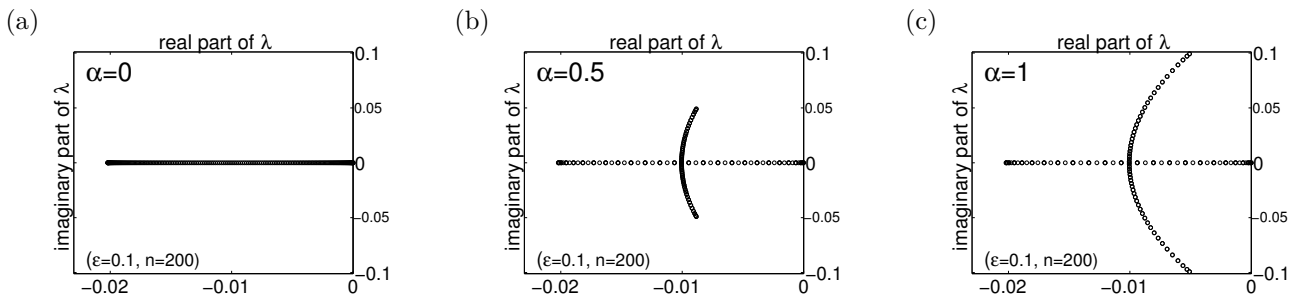
Figure 9: A plot of “slow” eigenvalues of matrix \mathcal{B} for n = 200 and \varepsilon = 0.1 . We plotted only eigenvalues close to zero for different strength of the signal \alpha from (3.27), namely: (a) \alpha = 0 , (b) \alpha = 0.5 and (c) \alpha = 1 .
