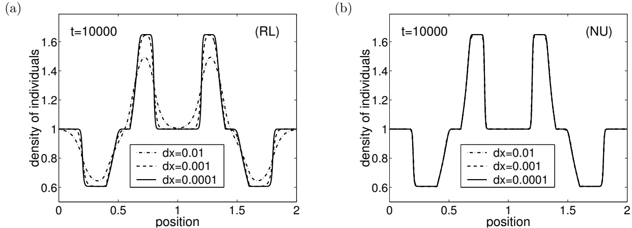
Figure 10: (a) Graph of a solution of (RL) given by \dot{w} = Aw at time t = 10^4 for different choices of \delta x . We used s = 0.0001 , signal given by (3.27) with \alpha = 0.1 , \delta t given by (4.19) and initial conditions (4.23). Consequently, \delta x = 0.01 , \delta x = 0.001 and \delta x = 0.0001 correspond to \varepsilon = 0.01 , \varepsilon = 0.1 , and \varepsilon = 1 , respectively. (b) Graph of a solution of (NU) given by \dot{z} = Bz at time t = 10^4 for different choices of \delta x . The parameters are the same as in (a).
