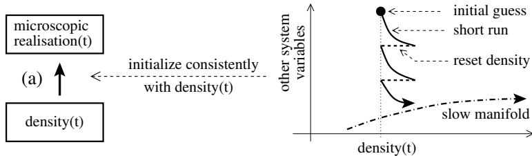
Figure 3: Initialization of other state variables in step (a).
