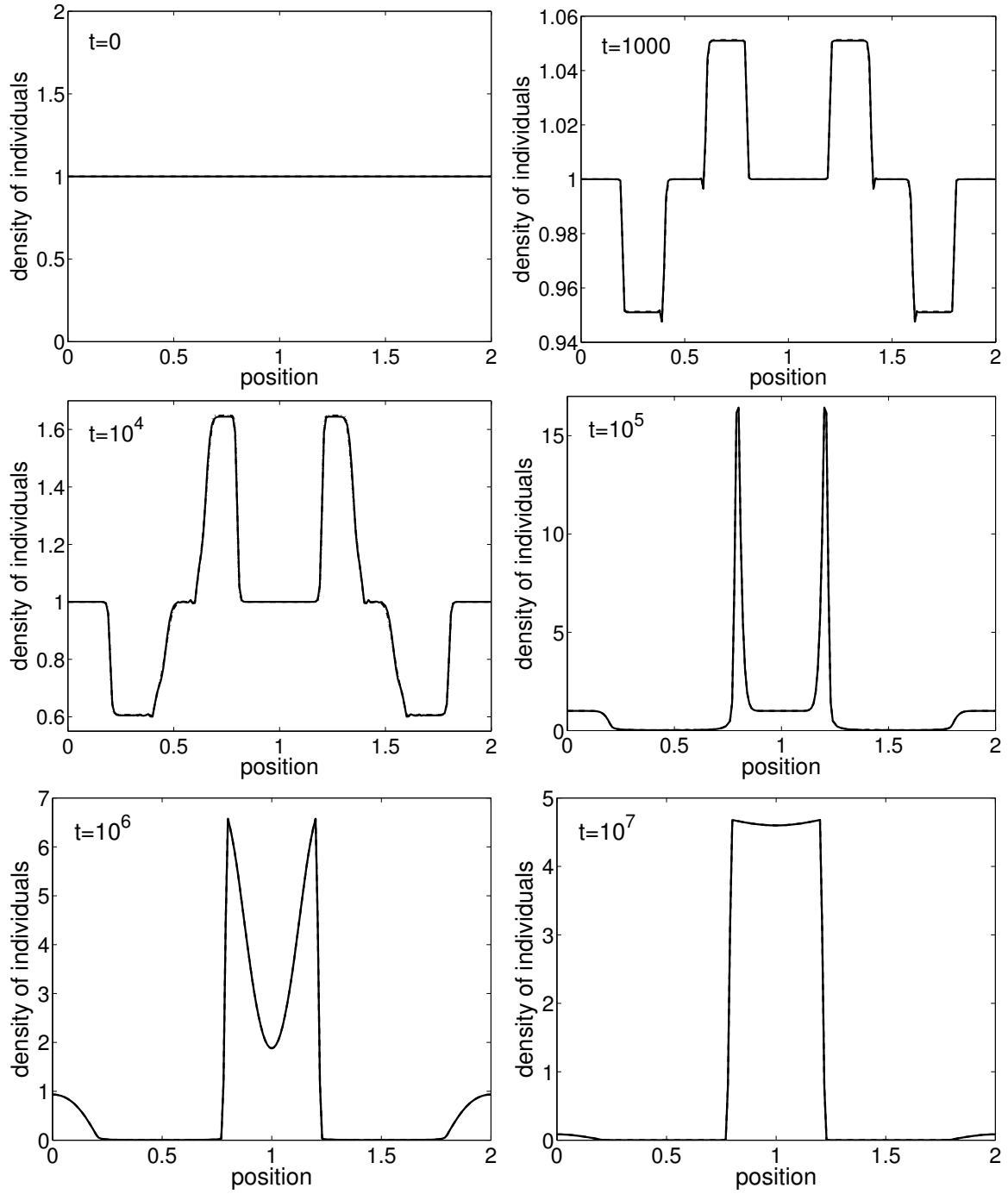
Figure 11: The time evolution of the density of individuals for s = 0.0001 and \alpha = 0.1 . We plot the solution of the system (4.16) (dashed line) and the solution obtained by the projective algorithm (P_k^M - 1) - (P_k^M - 3) for (4.16) with k = 1 and M = 398 (solid line). The gain \mathcal{G} is 200. We use (4.22), (4.19) and (4.23).
