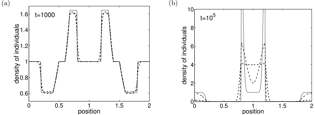
Figure 12: (a) Density of individuals for s = 0.0001 and \alpha = 1 at time t = 1000 . We plot the solution of (NJ) given by accurate numerical method (solid line), the solution obtained by projective algorithm (P_k^M - 1) - (P_k^M - 3) for (4.13) with (4.22), k = 1 and M = 198 , i.e., with \mathcal{G} = 100 (dashed line). We also plot the solution obtained by projective algorithm (P_k^M - 1) - (P_k^M - 3) for (4.13) with (4.24), k = 1 and M = 18 , i.e., with \mathcal{G} = 10 (dot-dashed line). In all computations, we use (4.19) and (4.23). (b) The same plots as in (a) for time t = 10^5 .
