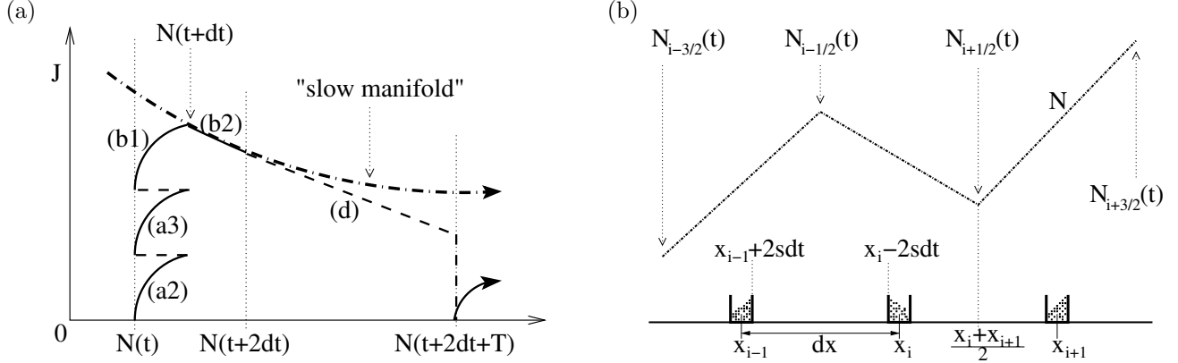
Figure 13: (a) Schematic of steps (a1) – (d) of the coarse integration algorithm. Monte Carlo simulation is denoted by solid lines. Dashed lines denote relatively fast steps, i.e., resetting the values of density to N(t) in steps (a2) and (a3) and the projective step (d). The dot-dashed line represents the evolution on the slow manifold of the system. We assume that the slow manifold can be accurately parametrized by density. (b) Schematic of three macroscopic mesh points x_{i-1} , x_i and x_{i+1} and kMC computational domains around them. Only particles close to the mesh points need be considered; the remaining particles will not leave/enter the interval [0, x_i] during steps (a1) – (b2) and consequently, they do not have to be simulated. At the top, is the (piecewise linear) estimated density profile which is used in step (a1). We place particles in the small computational domains that their number is consistent with this density profile.
