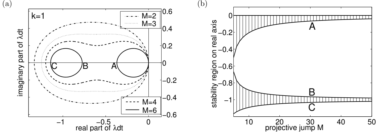
Figure 6: (a) The regions of absolute stability of P_k^M methods for k = 1 and M = 2 (dot-dashed line), M = 3 (dotted line), M = 4 (dashed line) and M = 6 (solid line). (b) Intersection of stability region from part (a) with real axis plotted as a function of M . The equations for boundary curves A(M) , B(M) and C(M) are given in Lemma 2.
