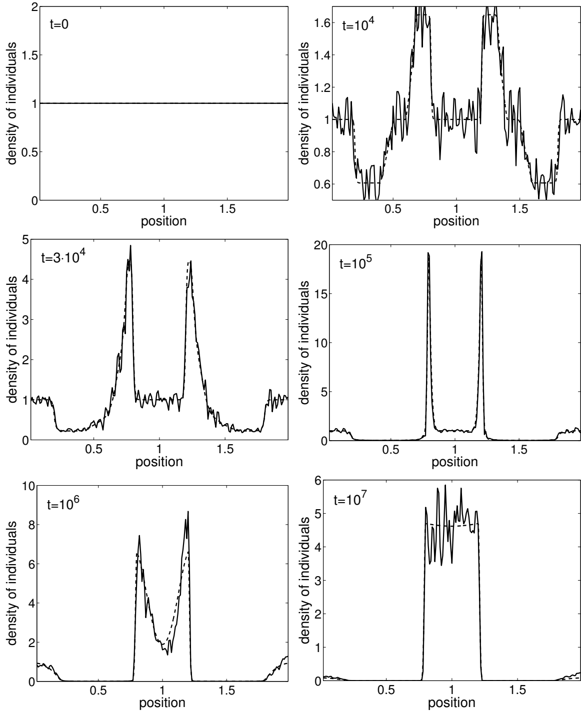
Figure 14: The time evolution of the density of individuals for (5.1), (5.5), \alpha = 0.1 and initial conditions (4.23). We plot the density given by coarse integration (a1) – (d) and obtained by formula (5.8) from the computed cumulative density function C(t) (solid line). Here we have gain \mathcal{G} = 1250 . We also plot the solution of the corresponding macroscopic moment equations (dashed line).
