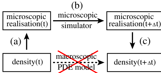
Figure 1: Schematic of microscopic timestepper (a) – (c).
