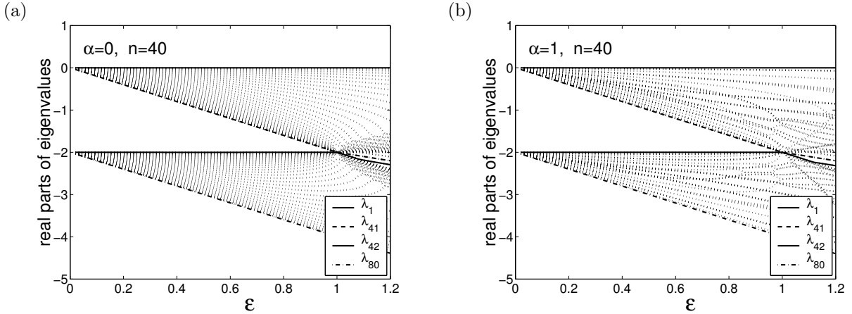
Figure 7: (a) Graph of real parts of eigenvalues of matrix \mathcal{A} for n = 40 and no signal gradient in the environment, i.e. , S'_0 = S'_1 = \dots S'_n = 0 . The eigenvalues are real for \varepsilon \in [0, 1] and there is a spectral gap between \lambda_{41} and \lambda_{42} . (b) Graph of real parts of eigenvalues of matrix \mathcal{A} for signal given by (3.27) with \alpha = 1 and for n = 40 .
