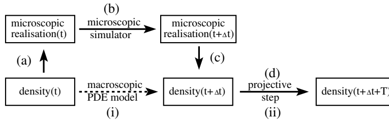
Figure 2: We first analyse (i) – (ii) in parameter regimes where macroscopic equations are available.
