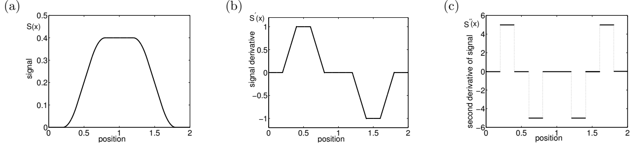
Figure 4: (a) Graph of “hat-profile” signal function \bar{S}(x) . (b) Graph of \bar{S}'(x) . (c) Graph of \bar{S}''(x) .
