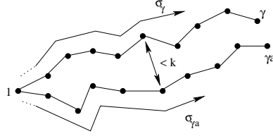
Figure 2. The fellow-traveller property
