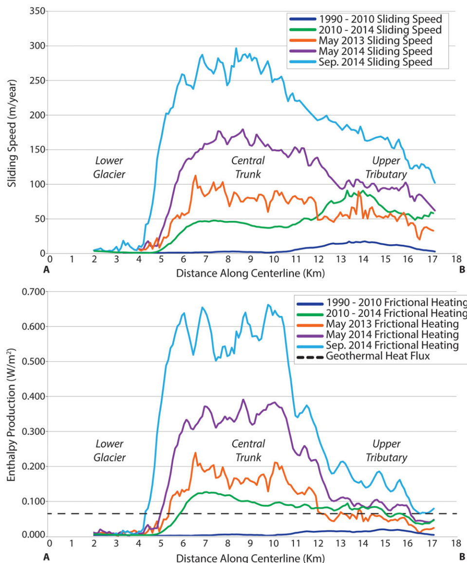
Fig. 12. Sliding velocities and enthalpy production rates 1990–2014.
