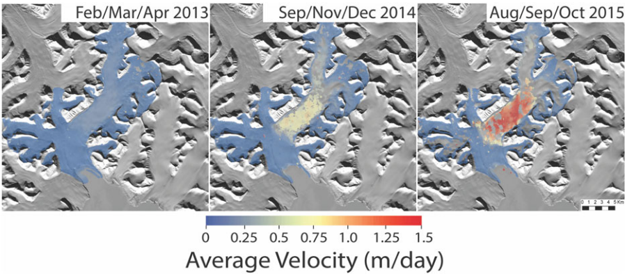
Fig. 7. Maps of time-averaged TerraSAR-X velocity data, showing the early evolution of the surge.
