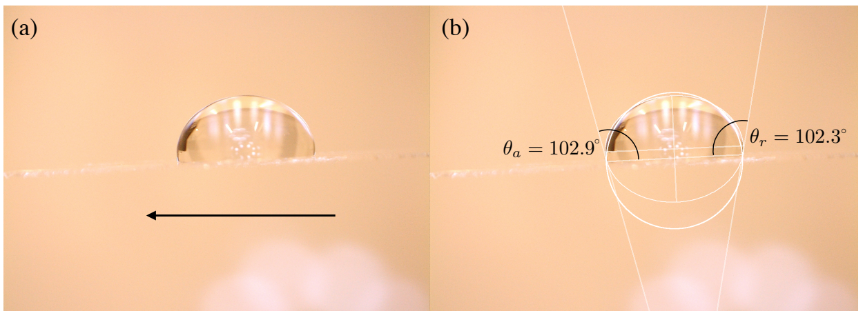
FIG. S2: Contact angle measurements of a Glycerol/Water Mix (GWM) droplet on a SLIPS infused with V5 silicon oil. (a) Image taken as a 15\ \mu\text{L} droplet slides down the surface, which is inclined by approximately 1^\circ to the horizontal. The black arrow indicates the direction of motion. (b) The same image with an elliptical fit applied to the drop using the contact angle plug-in in ImageJ. The angles measured in this image are \theta_a = 102.9^\circ and \theta_r = 102.3^\circ .
