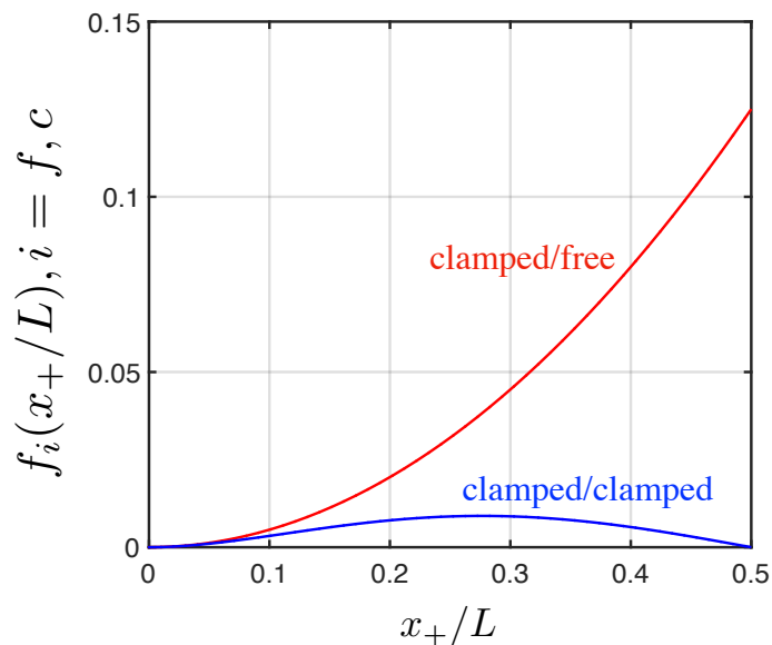
FIG. S5: The dimensionless meniscus speeds with the far end free or clamped cases f_i(x) , i = f, c , respectively, as defined in the main text. The meniscus speed for the clamped far end (blue curve) is significantly slower than that in with the free far end (red curve).
