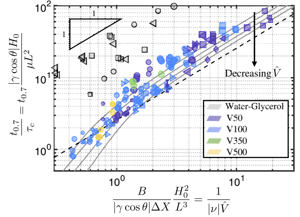
FIG. 3. Collapse of experimental data when rescaled according to Eq. (2). Points correspond to experimental observations (with volume and wall separation encoded by point size and shape, respectively, as in Fig. 2; droplet type is encoded by color, as indicated in the legend). The single set of error bars extends 1 standard deviation away from a particular data point, computed from 20 measurements, and is similar for each experiment [17]. Solid curves show results from numerical solutions of Eqs. (3)–(5) with \hat{V} = 0.5, 0.4, 0.3 and \hat{V} = 0.2 . Also plotted is the asymptotic result Eq. (7) (black dashed line), valid for \hat{V} \ll 1 (corresponding to the upper right corner of this plot).
