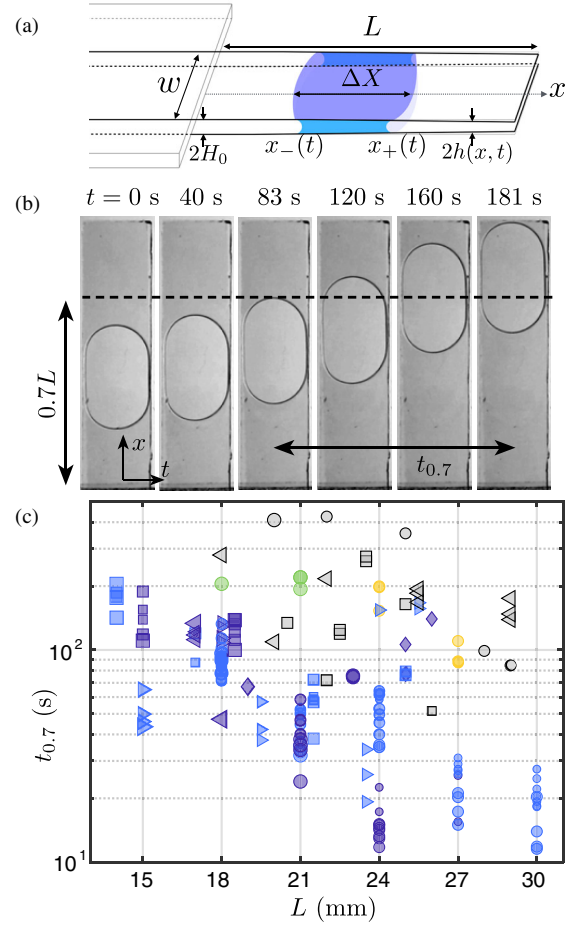
FIG. 2. (a) Schematic of a droplet in a flexible channel of undeformed wall separation 2H_0 , width w , and length L , with menisci positioned at x = x_-(t) and x = x_+(t) . (b) Top view of a droplet of V50 silicone oil (channel length L = 18 mm, width w = 5 mm, wall separation 2H_0 = 310 \mu\text{m} , thickness b = 300 \mu\text{m} , and droplet volume V = 10 \mu\text{L} ). Although the droplet spans the width of the channel, it is not precisely two dimensional. We present data for t_{0.7} , the time between the events x_+/L = 0.7 and x_+/L = 1 , which corresponds to the time between the third and sixth images here. (c) Raw experimental measurements of t_{0.7} , for different wall lengths, L . Data are shown for droplets of wetting silicone oil and a nonwetting water-glycerol mix; droplet type is encoded as in the legend of Fig. 3. Different shapes encode channel wall separation as follows: 2H_0 = 310 \mu\text{m} (right triangle), 360 \mu\text{m} (left triangle), 430 \mu\text{m} (square), 540 \mu\text{m} (circle), 630 \mu\text{m} (diamond). The size of each point encodes the approximate fraction of the channel taken by the droplet ( \hat{V} = \Delta X/L ), with bins corresponding to \hat{V} < 0.25 , 0.25 \leq \hat{V} < 0.35 , 0.35 \leq \hat{V} < 0.45 , and \hat{V} \geq 0.45 .
