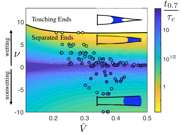
FIG. 4. Influence of dimensionless droplet volume \hat{V} and channel bendability \nu on the time taken to traverse the final 30% of the channel, t_{0.7}/\tau_c . Numerical results are shown by varying color, while the bold black curve indicates parameter values for which the edges of the channel touch during the motion, trapping the droplet. (Note that the position of this curve depends on the initial condition; here, x_+^0/L = 0.6 .) Positive bendability, \nu > 0 , corresponds to wetting drops, while \nu < 0 corresponds to nonwetting drops; when \nu = 0 , the channel is effectively rigid and the droplet remains stationary. Schematics illustrate typical configurations, and filled circles correspond to the experimental data presented in Figs. 2 and 3; the outliers with \nu < 0 are in the slow nonwetting regime.
