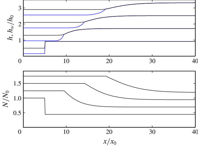
FIGURE 6. (Colour online) A region of underpressure upstream connected to a region of normal pressure downstream. The initial condition involves a jump in h and h_w at the junction between underpressure and normal pressure. Solutions are shown at times t/t_0 = 0, 5, 10, 15 with vertical offsets for N/N_0 of 0.05t/t_0 , and of 0.16t/t_0 for h/h_0 . The shock disappears and is replaced by an expansion fan in h_w on the underpressured side. Parameter values are q_- = 0.1q_0 , q_+ = 0.9q_0 , \varepsilon = 1 , p_i/N_0 = 1 .
