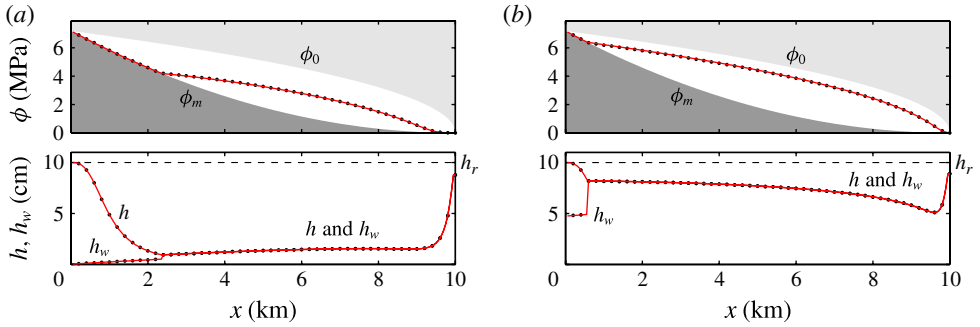
FIGURE 9. (Colour online) Steady-state solutions for a glacier with zero thickness at the upstream end, same line scheme as in figure 7. Both cases have m = 20 \text{ mm d}^{-1} , with inflow from upstream at: (a) q_n = 0 ; and (b) q_n = 0.01 \text{ m}^2 \text{ s}^{-1} .
