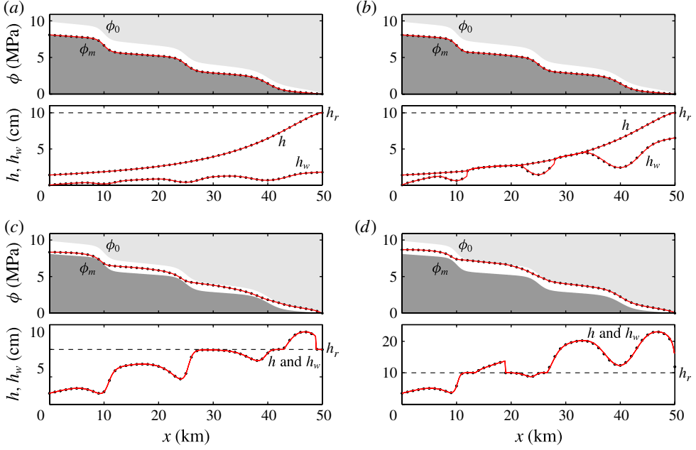
FIGURE 8. (Colour online) Steady-state solutions for a stepped glacier, same line scheme as in figure 7: (a) m = 1 \text{ mm d}^{-1} ; (b) m = 5 \text{ mm d}^{-1} ; (c) m = 20 \text{ mm d}^{-1} ; (d) m = 40 \text{ mm d}^{-1} . q_n = 0 in all cases.
