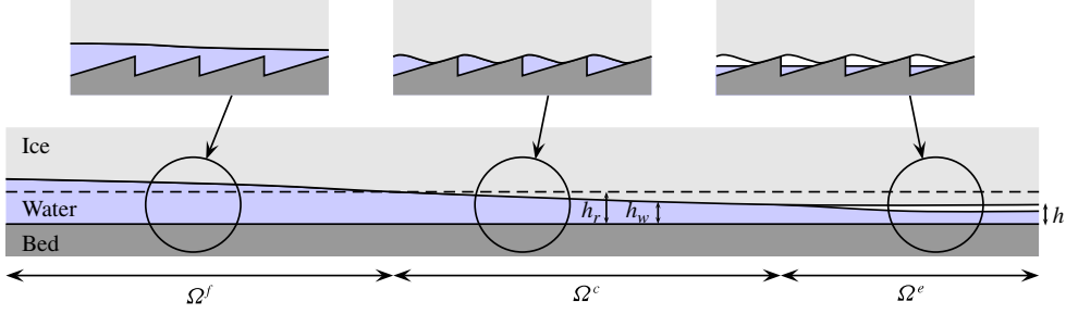
FIGURE 3. (Colour online) The partitioning of the domain \Omega into \Omega^e , \Omega^f and \Omega^c . Here h_r denotes the height of bed bumps, h is the mean void space height between ice and bed (averages over the bed roughness scale shown in the inset images), and h_w is the mean water depth at the bed, likewise averaged.
