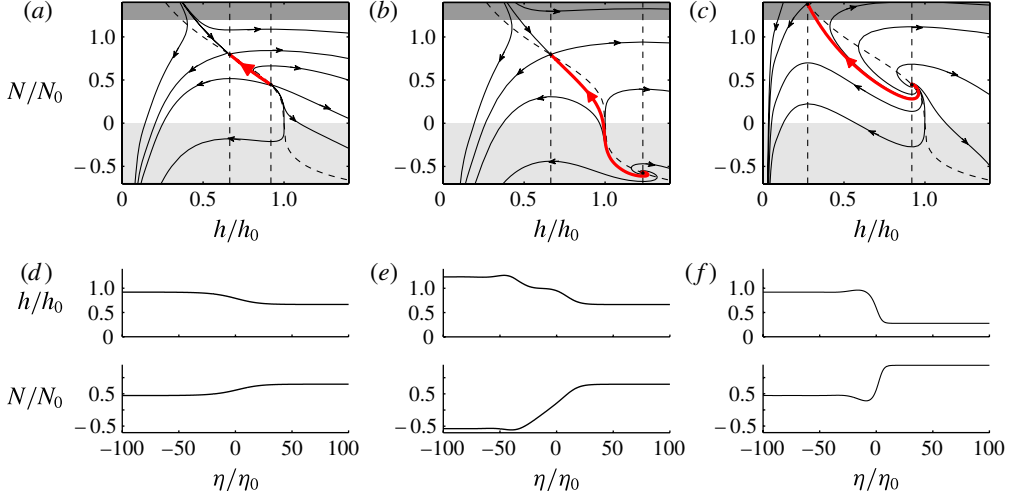
FIGURE 2. (Colour online) Travelling wave solutions. In these computations, we have used (2.5), and scaled the variables with h_0 = h_r , q_0 = kh_r^\alpha \Psi_0^{\beta-1} , N_0 = (u_b/\tilde{A}l_r)^{1/n} , \eta_0 = N_0/\Psi_0 , V_0 = q_0/h_0 . We then have a three-parameter family of solutions, determined solely by the scaled upstream and downstream fluxes q_+ and q_- and the length scale ratio \varepsilon = u_b\eta_0/(V_0l_r) . Here we have put \varepsilon = 0.25 . The top row, (a–c), shows the phase plane, and the bottom row, (d–f), the actual travelling wave solutions h(\eta) and N(\eta) . In each phase portrait, the dashed lines are nullclines, while the thick orbit (shown in red in the online version) is the unique orbit connecting the two fixed points. The light grey and dark grey shaded regions represent N < 0 and N > p_i respectively, where we have arbitrarily set p_i = 1.2N_0 here. (a,d) ( q_- = 0.9q_0 and q_+ = 0.6q_0 ) correspond to a physically acceptable solution, in which N never becomes negative or exceeds the ice overburden p_i ; (b,e) ( q_- = 1.3q_0 and q_+ = 0.3q_0 ) show a solution in which effective pressure becomes negative and gap width h exceeds the roughness scale h_r sufficiently far upstream; (c,f) ( q_- = 0.9q_0 and q_+ = 0.2q_0 ) show a solution for which N > p_i sufficiently far downstream.
