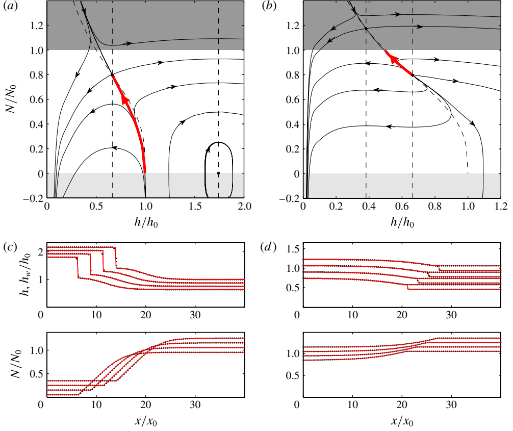
FIGURE 5. (Colour online) Travelling wave solutions with over- and underpressured regions. We have used the same scales as in figure 2, which now yield a three-parameter family of solutions, determined by the scaled fluxes q_+ and q_- , the length scale ratio \varepsilon , and the scaled overburden p_i . Here we set \varepsilon = 1 and p_i/N_0 = 1 . The top row, (a,b), shows the phase plane with the same layout as in figure 2. The bottom plots, (c,d), show the actual travelling wave solutions h(x, t) (as well as h_w(x, t) where this differs from h(x, t) ) and N(x, t) at different times. For clarity, the solutions for h/h_0 are offset vertically at different times by amounts 0.06t/t_0 and 0.08t/t_0 in (c) and (d), respectively, where t_0 = \eta_0/V_0 . The solutions for N/N_0 are offset by 0.05t/t_0 in both plots. Solutions are plotted for t/t_0 = 1, 3, 5, 7 . Where there are two lines in the plots of h and h_w , the lower one represents h_w in an underpressured region. The solid lines in (c,d) (red in the online version) correspond to the solution computed from phase-plane analysis using an ordinary differential equation solver, while the dots show the solution computed numerically using the method in §4.3. (a,c) A solution with overpressure upstream ( q_- = 0.6q_0 and q_+ = 0.3q_0 ); (b,d) underpressure downstream ( q_- = 2q_0 and q_+ = 0.5q_0 ).
