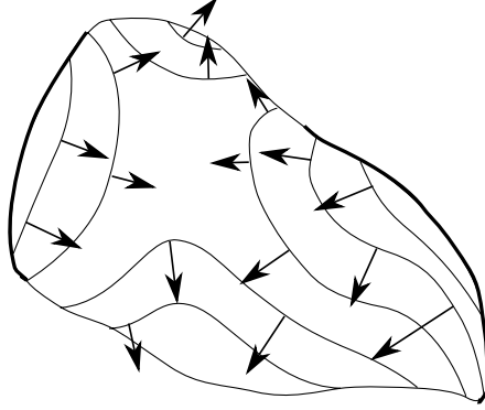
FIGURE 4. Identification of inflow and outflow boundaries. Contour lines of \phi_0 (or \phi_m ) are shown with arrows pointing from high \phi_0 to low \phi_0 . The parts of the boundary marked as thick curves are then \phi_0 - (or \phi_m -) inflow boundaries, while the remaining parts are \phi_0 - (or \phi_m -) outflow boundaries.
