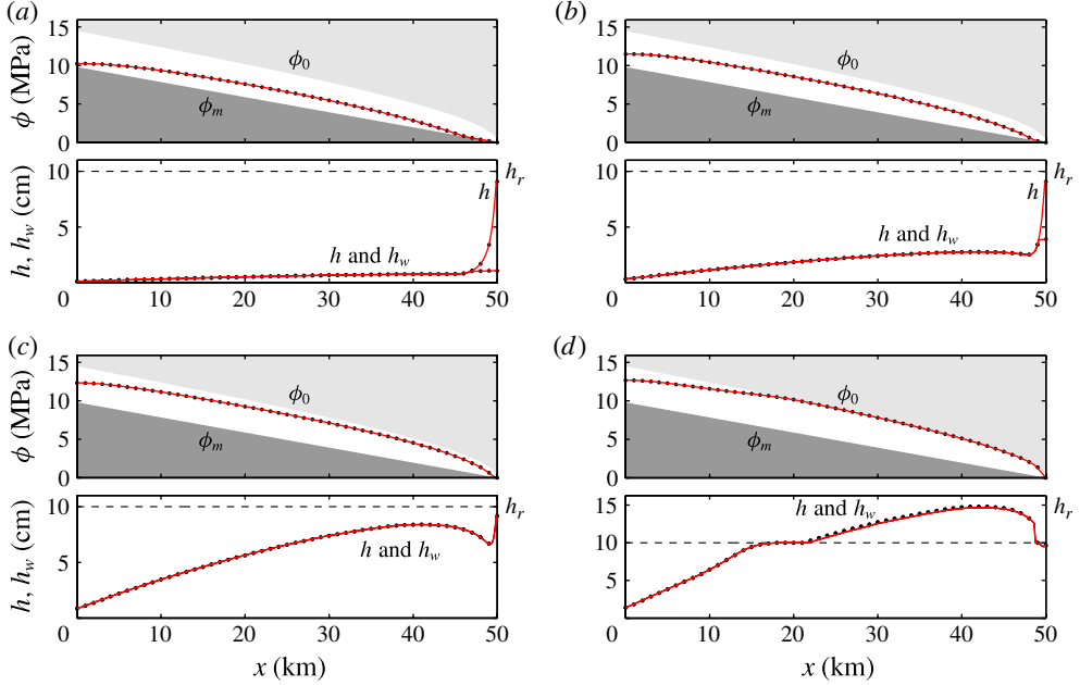
FIGURE 7. (Colour online) Steady-state solutions for a plastic glacier. Each pair of plots corresponds to a different value of m : (a) m = 1 \text{ mm d}^{-1} ; (b) m = 5 \text{ mm d}^{-1} ; (c) m = 20 \text{ mm d}^{-1} ; (d) m = 40 \text{ mm d}^{-1} . q_n = 0 in each case. The top plot each pair shows \phi(x) computed from (5.13) as a solid line (red in the online version), with dots marking the numerical solution computed using the method in § 4.3. The ‘forbidden’ regions \phi < \phi_m and \phi > \phi_0 are shaded in dark and light grey, respectively. Over- and underpressure occur where the solution \phi(x) coincides with the boundaries of these regions. The bottom plot in each pair shows h(x) and, if different, h_w(x) below the curve for h(x) (both red in the online version). In other words, cavities are partially air-filled where the solid line splits in two, as is the case in the m = 1 \text{ mm d}^{-1} case (a) at 45 km. The horizontal dashed line in the bottom plot of each pair corresponds to the mean obstacle height h_r , so that complete bed separation occurs when the solid line representing h rises above the dashed line, as is the case in the m = 40 \text{ mm d}^{-1} case (d) at 25 km. As before, solid lines show the solution computed from (5.13), and dots the solution obtained from § 4.3, and we observe close agreement.
