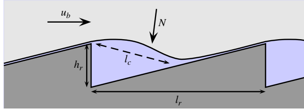
FIGURE 1. (Colour online available at journals.cambridge.org/flm ) A single cavity.
