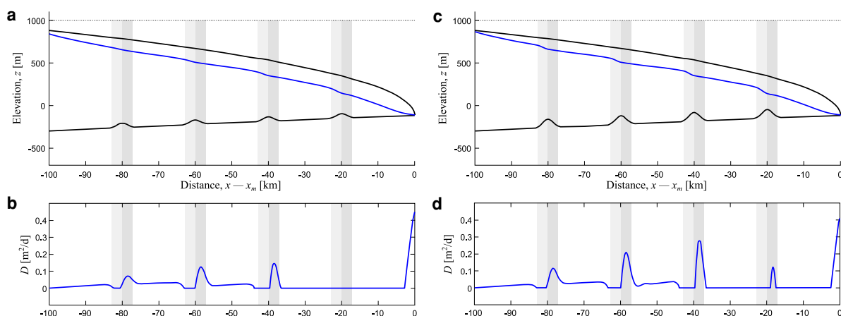
Fig. 3. Deposition over Gaussian ridges, placed at 20, 40, 60 and 80 km from the ice margin. Panels (a) and (c) show the ice and bed geometry, while panels (b) and (d) plot the sediment deposition rate. Ridges of 50 m amplitude are considered in (a) and (b). Note that deposition does not occur at the 20 km ridge. For the 100 m amplitude ridges shown in (c) and (d), deposition rates are higher overall, and deposition does occur at the ridge situated 20 km from the ice margin.
