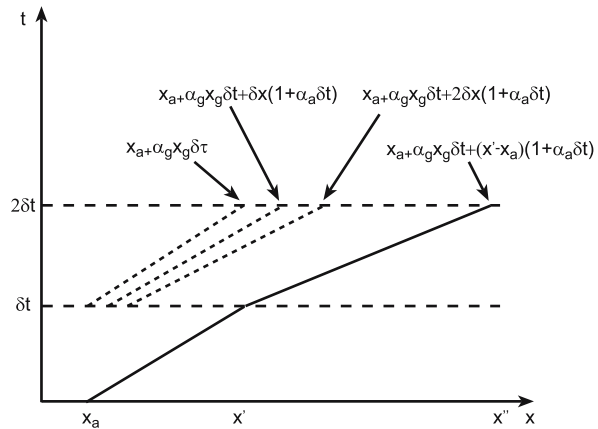
Fig. 8 The solution from ‘first principles’. Over the first time step \delta t , the point x_a is mapped to x_a + \alpha_g x_g \delta t . The region [x', x_a] is then divided into N intervals of width \delta x ; over the time step \delta t each one grows to fill a region of width \delta x(1 + \alpha_a \delta t) etc
