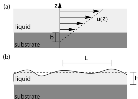
Figure 1. (a) Illustration of hydrodynamic slip: liquid flows along a substrate (the arrows indicate the flow field u(z) ). In systems with slip, the flow velocity at the liquid–substrate interface is not zero. The flow velocity as a function of z extrapolated into the substrate (dashed line) is zero at a depth b called the slip length. (b) Fluctuations of the liquid surface in a spinodally dewetting thin film having a characteristic wavelength L . In the systems under consideration, this wavelength is large as compared to the initial/mean film thickness H .
