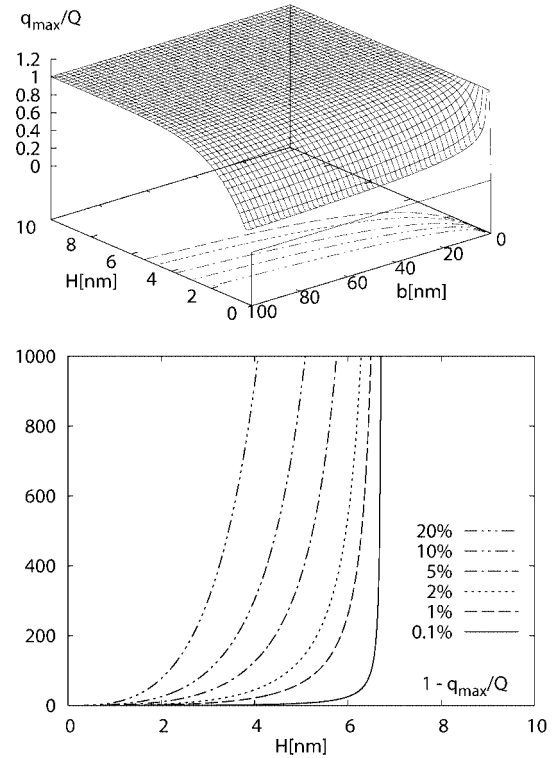
Figure 4. Shift of the position of the maximum q_{\max} of the dispersion relation \omega(q) as compared to the position expected for the weak and intermediate slip model and experimental parameters for a PS film on OTS from ref 7 as a function of the film thickness H and the slip length b . The contour lines indicate the slip length b necessary in order to obtain a deviation of 0.1%, 1%, 5%, 10%, and 20%.
