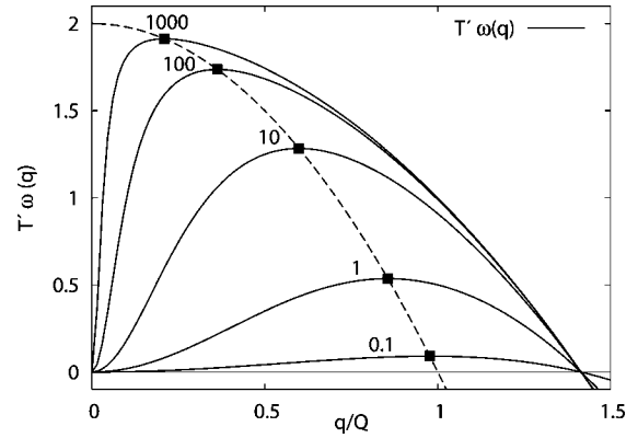
Figure 2. Dispersion relation in the strong-slip limit in eq 9 (full lines) for various values of B (indicated by the labels). The location of the maxima (boxes and dashed line) shifts to smaller values q/Q and the height approaches 2/T' from below for increasing B .
