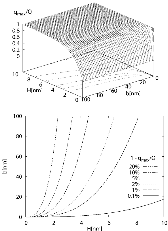
Figure 3. Shift of the position of the maximum q_{\max} of the dispersion relation \omega(q) as compared to the position expected for the weak- and intermediate-slip model and experimental parameters from ref 6 as a function of the film thickness H and the slip length b . The contour lines indicate the slip length b necessary in order to obtain a deviation of 0.1%, 1%, 5%, 10%, and 20%.
