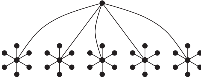
Fig. 5.8. Yet another tree Z_4 (Example 2.9 of [8] with k = 4 ) that has an eigenvalue exactly equal to 4. This is non-isomorphic to any tree spanned by vertex disjoint copies of K_{1,3} such as the one shown in Fig. 5.6(a).
