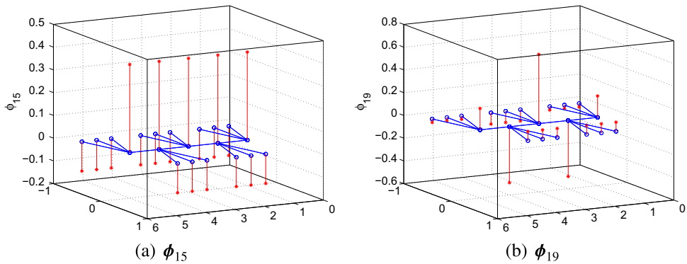
Fig. 5.7. (a) The eigenvector \phi_{15} corresponding to \lambda_{15} = 4 in the 3D perspective view. (b) The eigenvector \phi_{19} corresponding to the maximum eigenvalue \lambda_{19} = 7.1091 , which concentrates around the central vertex.
