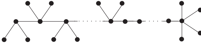
Fig. 7.9. Counterexample graph for the conjecture.
