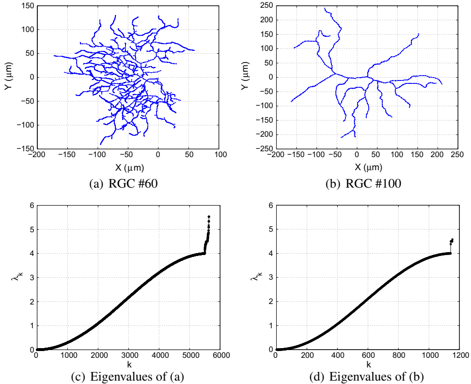
Fig. 1.1. Typical dendrites of retinal ganglion cells (RGCs) of a mouse and the graph Laplacian eigenvalue distributions. (a) 2D projection of dendrites of an RGC of a mouse; (b) that of another RGC revealing different morphology; (c) the eigenvalue distribution of the RGC shown in (a); (d) that of the RGC shown in (b). Regardless of their morphological features, a phase transition occurs at the eigenvalue 4.
