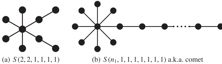
Fig. 3.4. Typical examples of a starlike tree.
