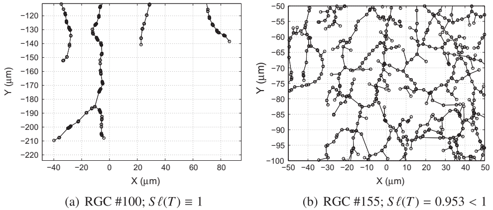
Fig. 4.5. Zoomed-up versions of parts of some dendritic trees.
