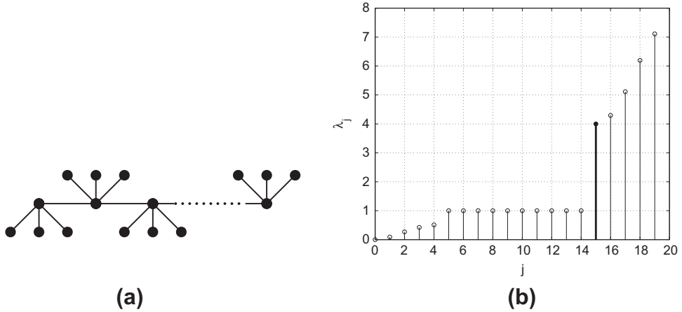
Fig. 5.6. (a) A tree spanned by multiple copies of K_{1,3} connected via their central vertices. This tree has an eigenvalue equal to 4 with multiplicity 1. (b) The eigenvalue distribution of such a tree spanned by 5 copies of K_{1,3} . We note that S\ell(T) = 1 for this tree.
