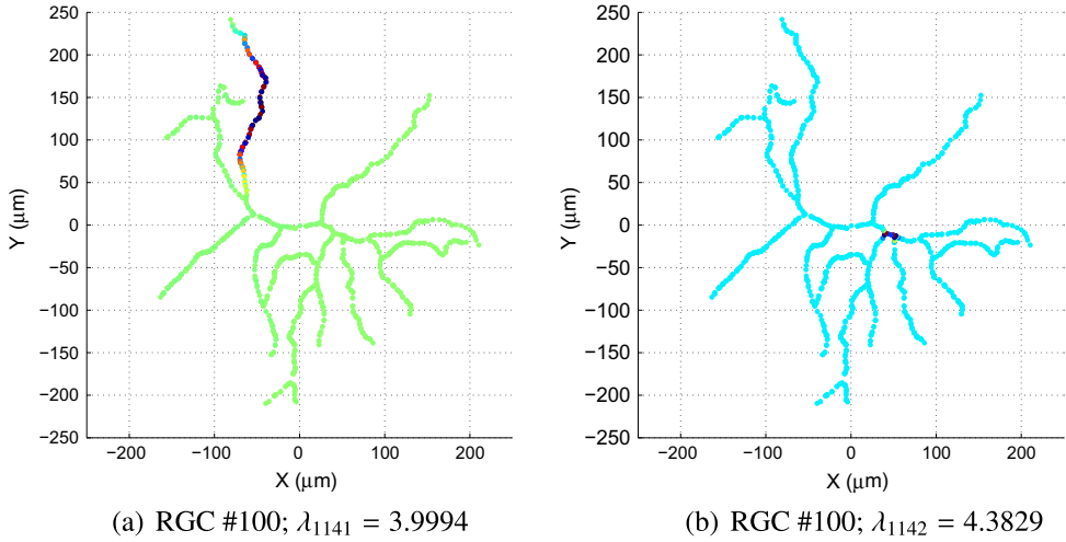
Fig. 1.2. The graph Laplacian eigenvectors of RGC #100. (a) The one corresponding to the eigenvalue \lambda_{1141} = 3.9994 , immediately below the value 4; (b) the one corresponding to the eigenvalue \lambda_{1142} = 4.3829 , immediately above the value 4.
