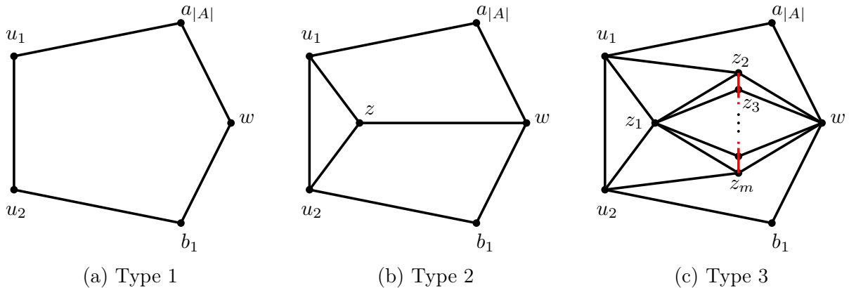
Figure 4: The possible configurations of vertices in F_1
