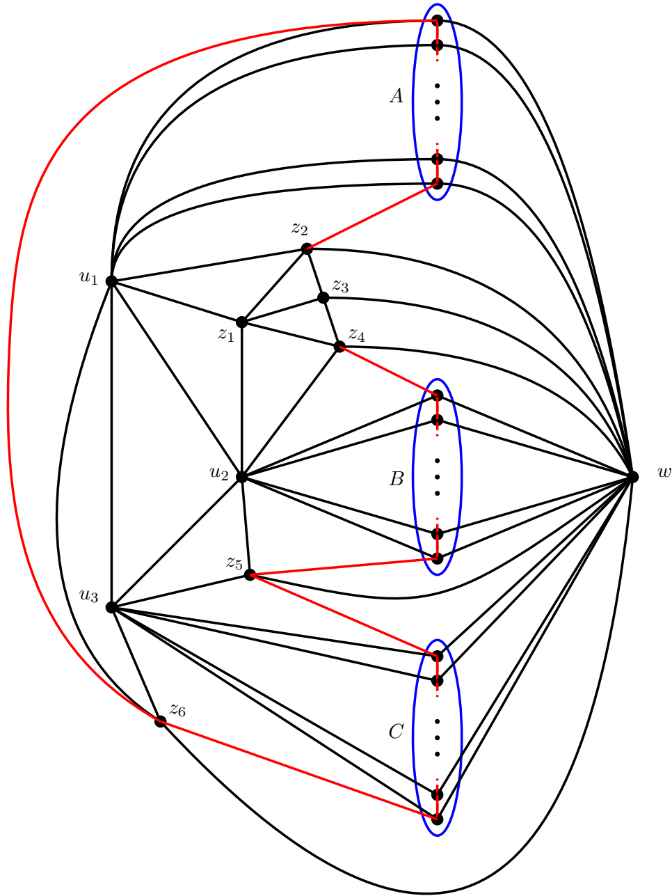
Figure 1: A graph of the required form
