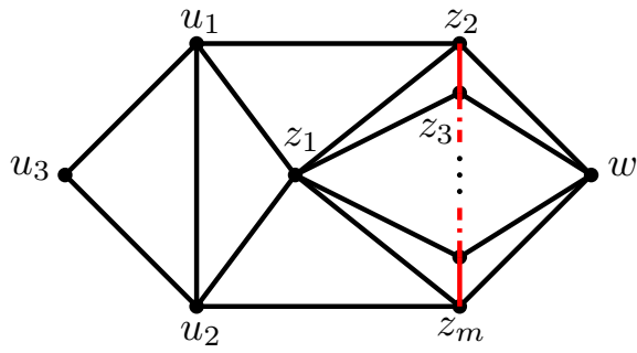
(a) H[\{u_1, u_2, u_3, w\} \cup Z_1] if F_1 is of type 3
