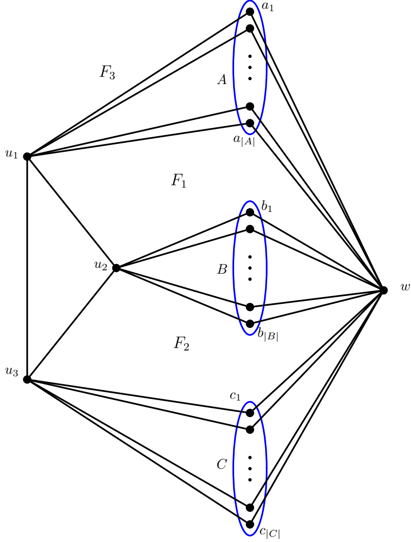
Figure 3: Illustration of the drawing of H - Z , with faces F_1 , F_2 , and F_3 labelled
