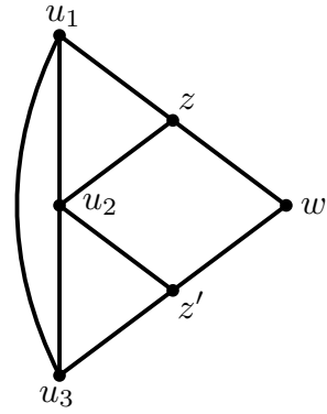
(b) H[\{u_1, u_2, u_3, w\} \cup Z_1 \cup Z_2] if F_1 and F_2 are both of type 2
