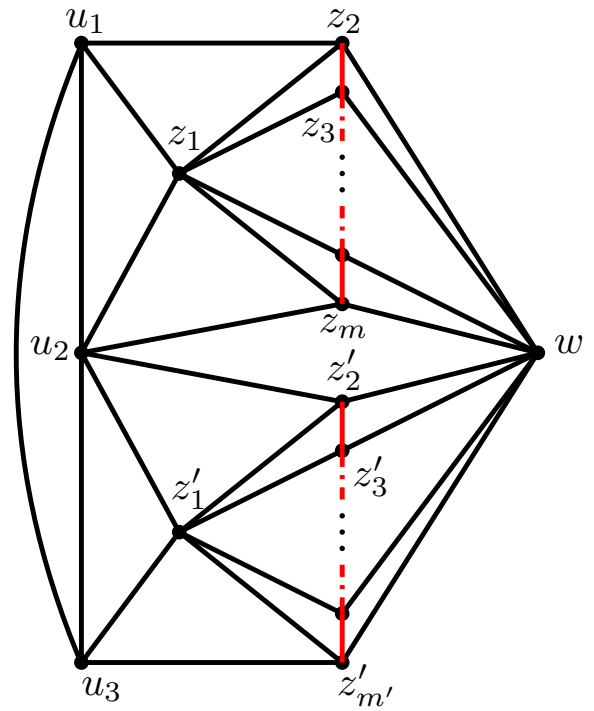
(d) H[\{u_1, u_2, u_3, w\} \cup Z_1 \cup Z_2] if F_1 and F_2 are both of type 3
