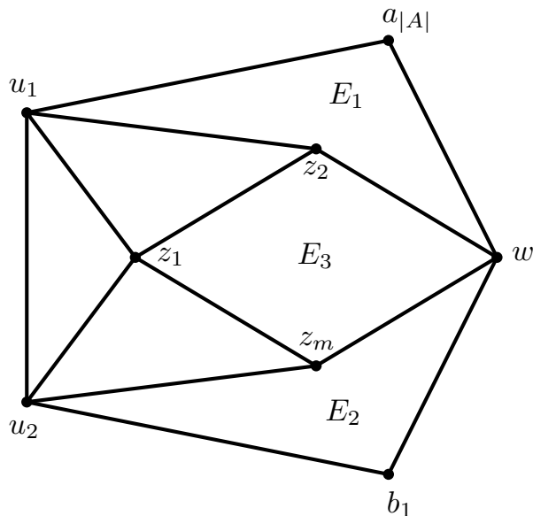
Figure 5: Illustration of the drawing of H[\{u_1, u_2, w, a_{|A|}, b_1, z_1, z_2, z_m\}] with the edge z_2 z_m deleted if present
