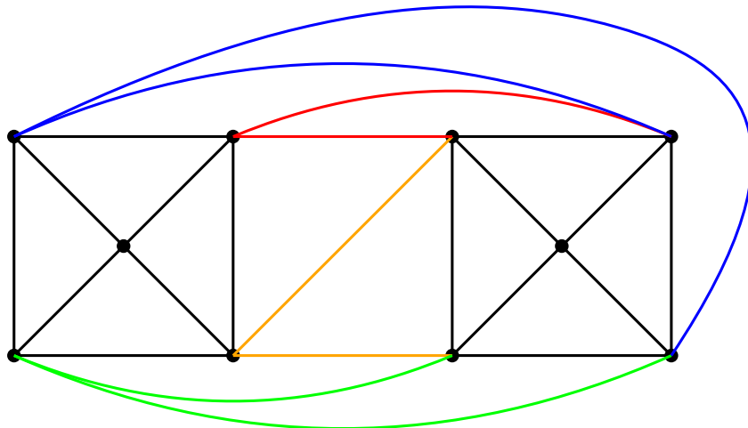
Figure 2: A planar graph with 10 vertices and 16 induced 5-cycles
